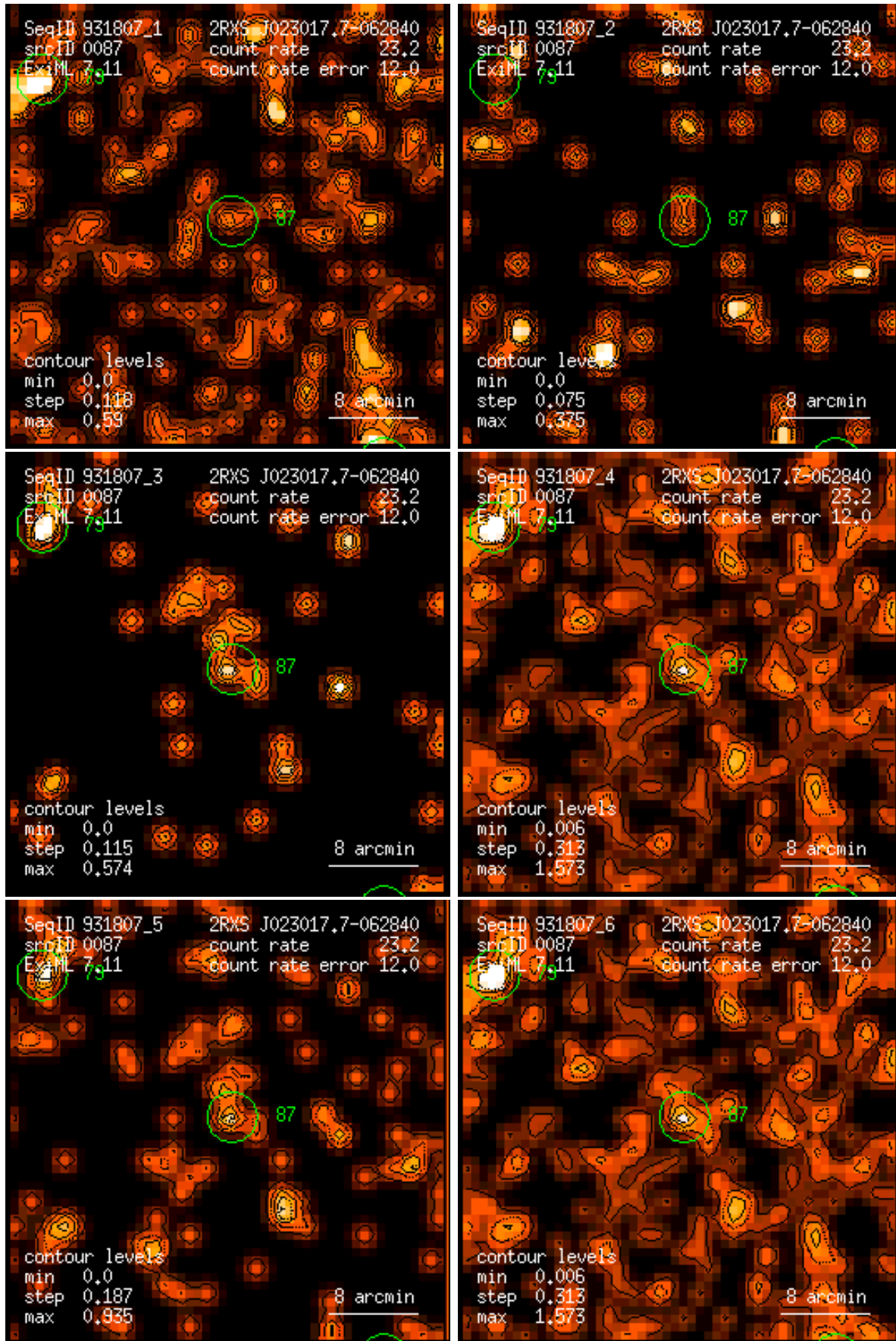
Figure 87: RASS 931807: detection 0087: band rate images, Gaussian filter: (1) PSPC channels 11 – 41, (2) 52 – 90, (3) 91 – 201, (4) 11 – 235, (5) 52 – 201, (6) 11 – 201. Broad band rates in counts/ks. Band rate contour levels in counts/ks/arcmin 2 .
