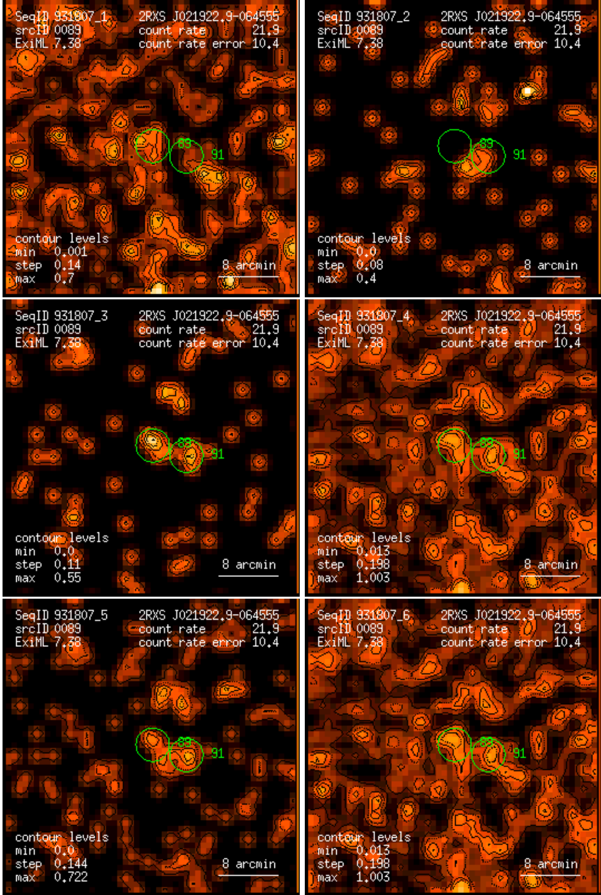
Figure 89: RASS 931807: detection 0089: band rate images, Gaussian filter: (1) PSPC channels 11 – 41, (2) 52 – 90, (3) 91 – 201, (4) 11 – 235, (5) 52 – 201, (6) 11 – 201. Broad band rates in counts/ks. Band rate contour levels in counts/ks/arcmin 2 .
