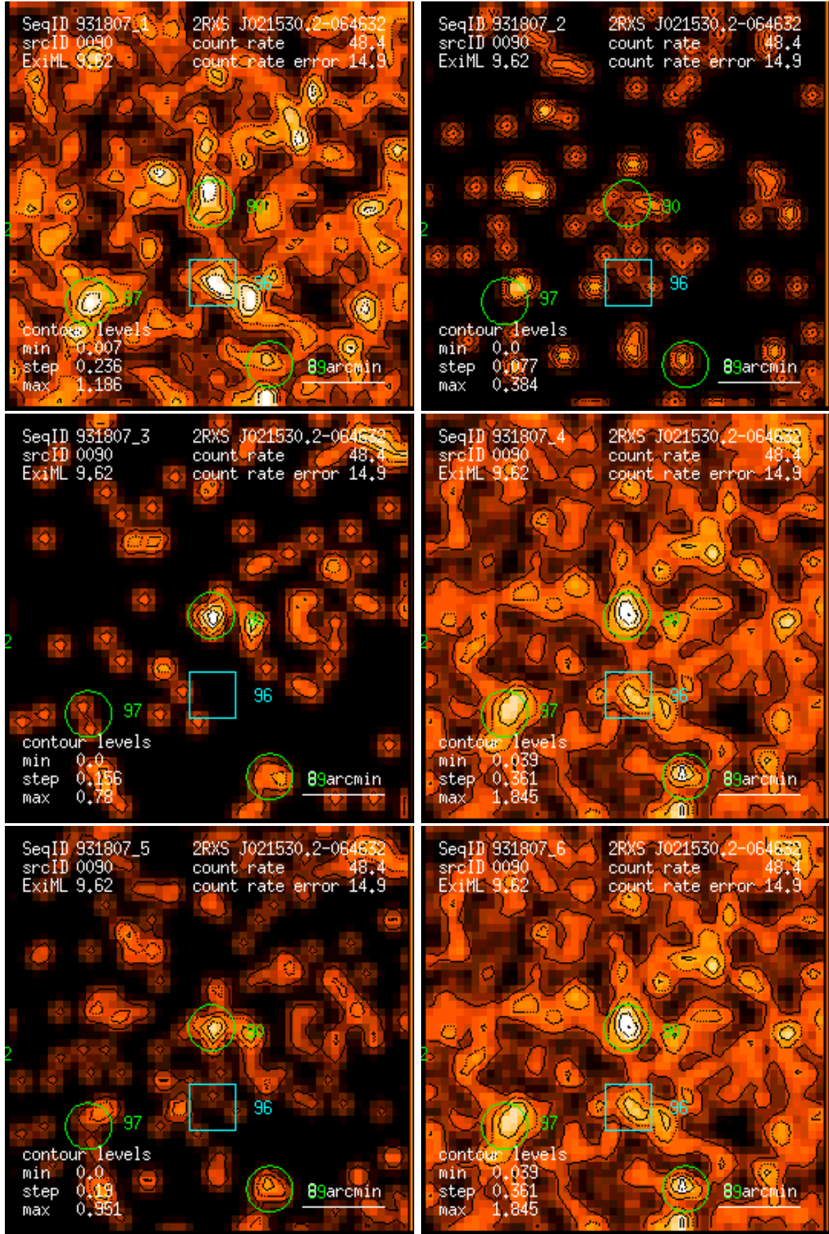
Figure 90: RASS 931807: detection 0090: band rate images, Gaussian filter: (1) PSPC channels 11 – 41, (2) 52 – 90, (3) 91 – 201, (4) 11 – 235, (5) 52 – 201, (6) 11 – 201. Broad band rates in counts/ks. Band rate contour levels in counts/ks/arcmin 2 .
