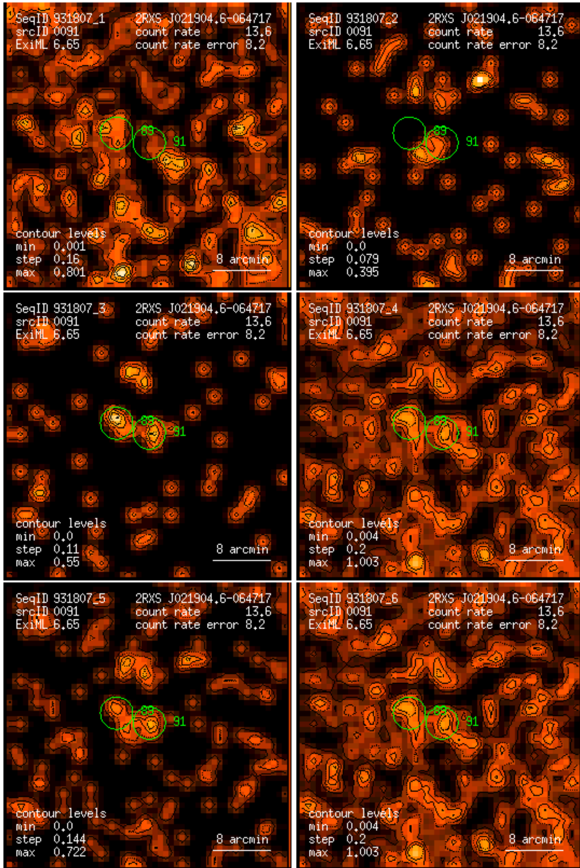
Figure 91: RASS 931807: detection 0091: band rate images, Gaussian filter: (1) PSPC channels 11 – 41, (2) 52 – 90, (3) 91 – 201, (4) 11 – 235, (5) 52 – 201, (6) 11 – 201. Broad band rates in counts/ks. Band rate contour levels in counts/ks/arcmin 2 .
