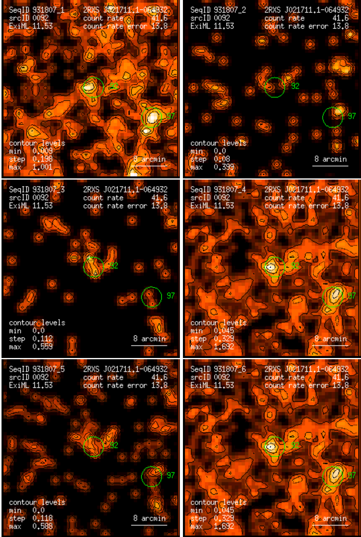
Figure 92: RASS 931807: detection 0092: band rate images, Gaussian filter: (1) PSPC channels 11 – 41, (2) 52 – 90, (3) 91 – 201, (4) 11 – 235, (5) 52 – 201, (6) 11 – 201. Broad band rates in counts/ks. Band rate contour levels in counts/ks/arcmin 2 .
