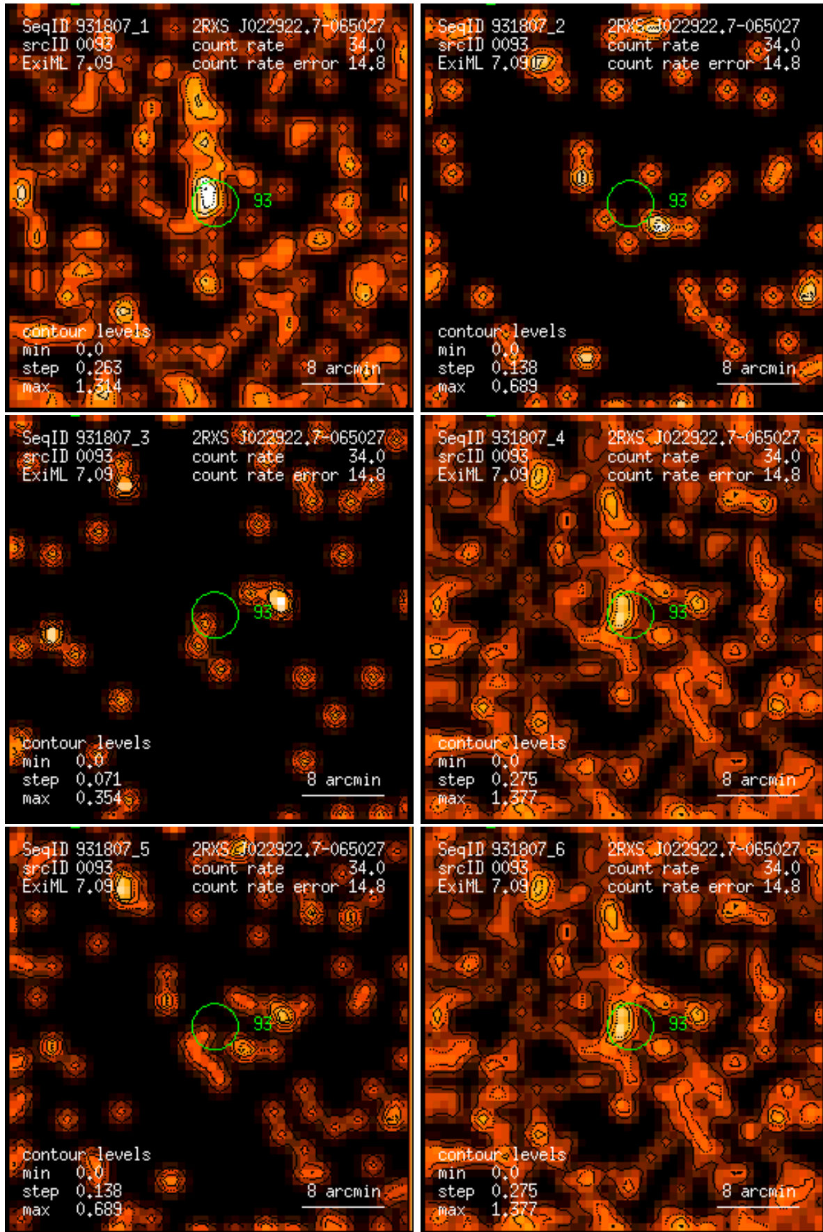
Figure 93: RASS 931807: detection 0093: band rate images, Gaussian filter: (1) PSPC channels 11 – 41, (2) 52 – 90, (3) 91 – 201, (4) 11 – 235, (5) 52 – 201, (6) 11 – 201. Broad band rates in counts/ks. Band rate contour levels in counts/ks/arcmin 2 .
