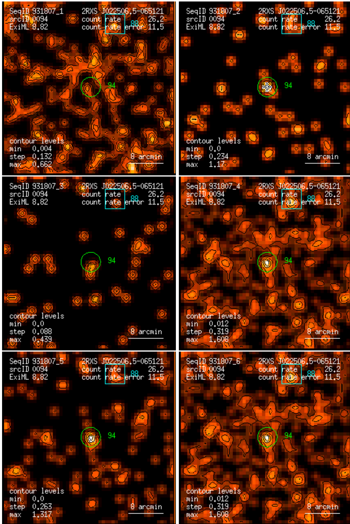
Figure 94: RASS 931807: detection 0094: band rate images, Gaussian filter: (1) PSPC channels 11 – 41, (2) 52 – 90, (3) 91 – 201, (4) 11 – 235, (5) 52 – 201, (6) 11 – 201. Broad band rates in counts/ks. Band rate contour levels in counts/ks/arcmin 2 .
