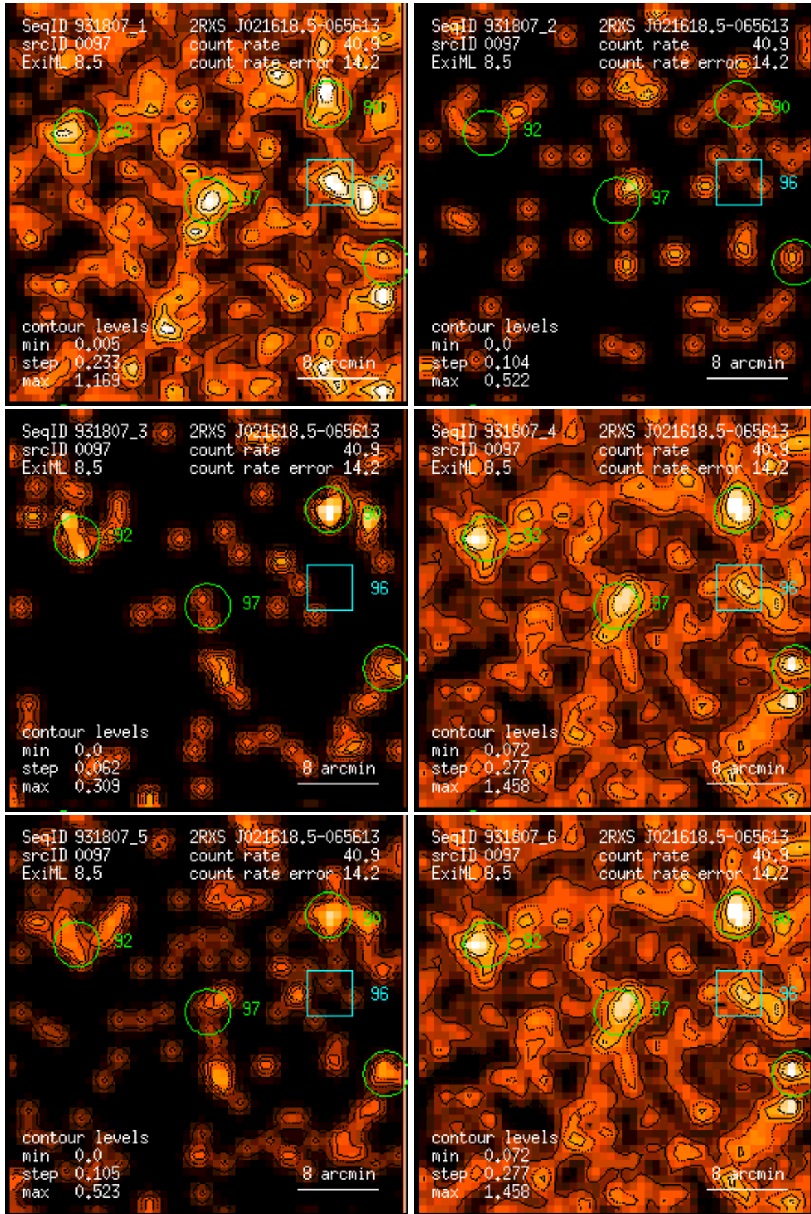
Figure 97: RASS 931807: detection 0097: band rate images, Gaussian filter: (1) PSPC channels 11 – 41, (2) 52 – 90, (3) 91 – 201, (4) 11 – 235, (5) 52 – 201, (6) 11 – 201. Broad band rates in counts/ks. Band rate contour levels in counts/ks/arcmin 2 .
