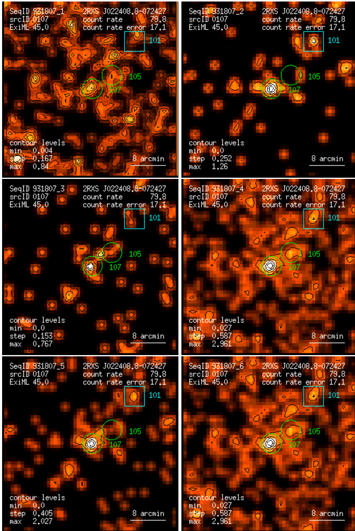
Figure 107: RASS 931807: detection 0107: band rate images, Gaussian filter: (1) PSPC channels 11 – 41, (2) 52 – 90, (3) 91 – 201, (4) 11 – 235, (5) 52 – 201, (6) 11 – 201. Broad band rates in counts/ks. Band rate contour levels in counts/ks/arcmin 2 .
