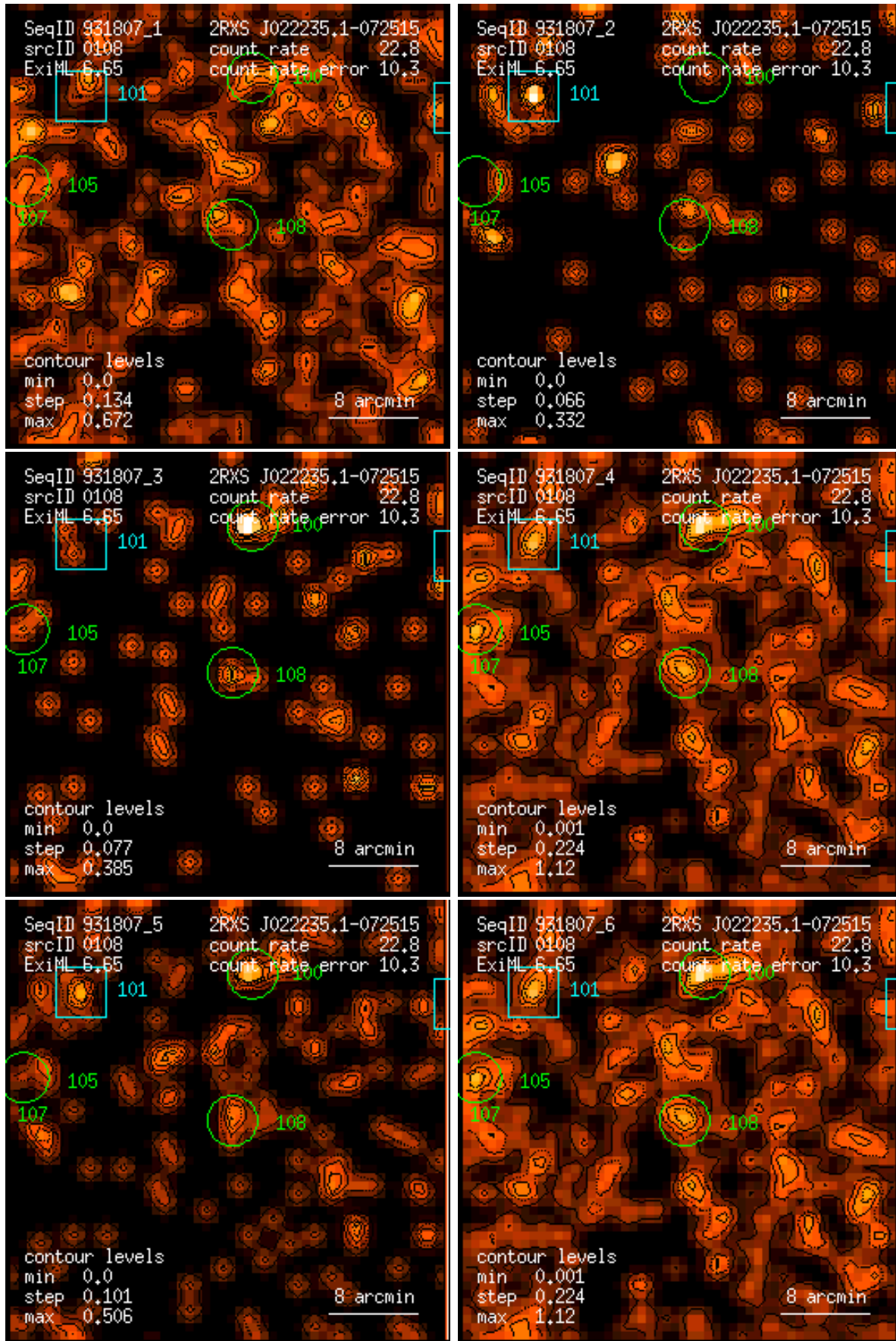
Figure 108: RASS 931807: detection 0108: band rate images, Gaussian filter: (1) PSPC channels 11 – 41, (2) 52 – 90, (3) 91 – 201, (4) 11 – 235, (5) 52 – 201, (6) 11 – 201. Broad band rates in counts/ks. Band rate contour levels in counts/ks/arcmin 2 .
