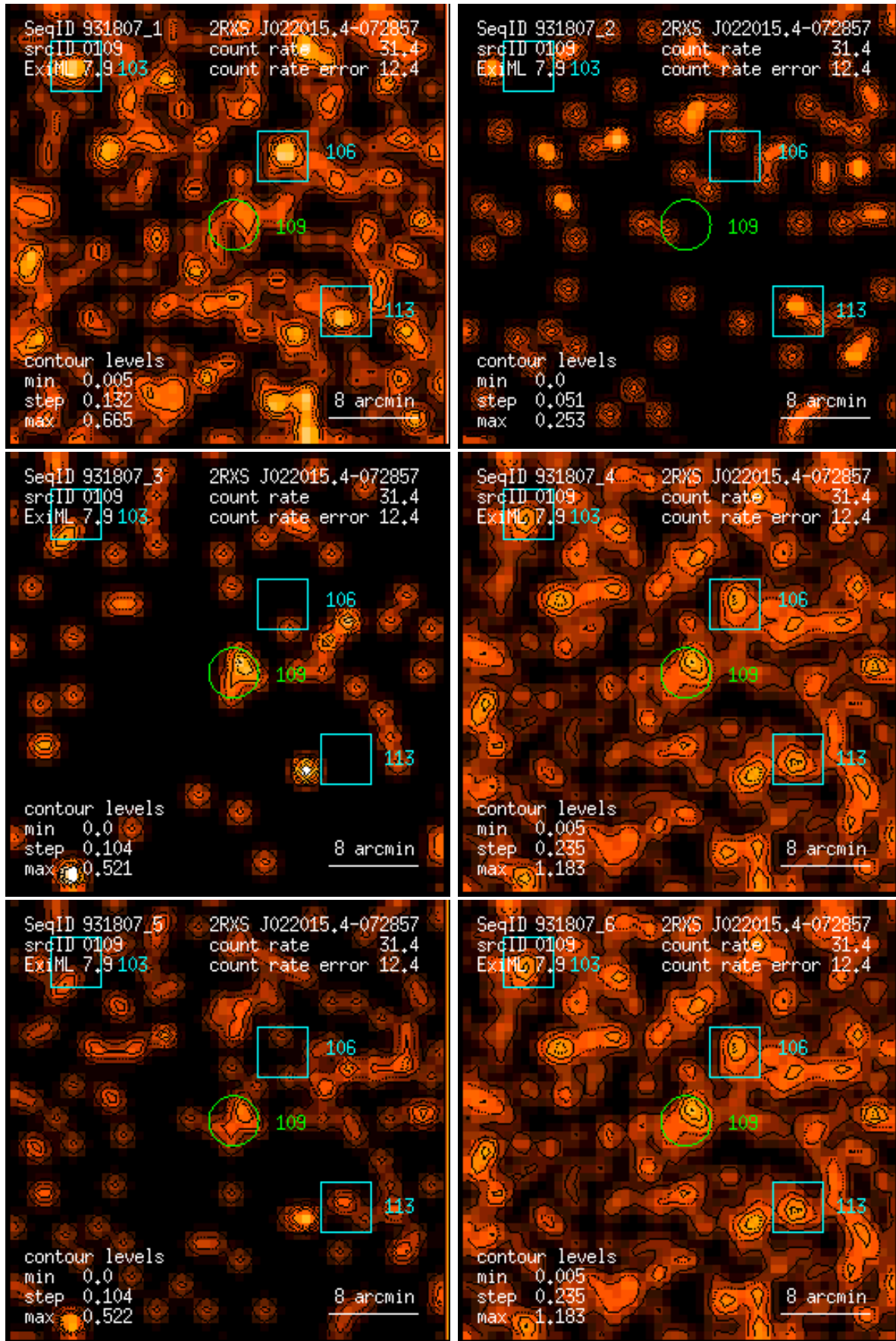
Figure 109: RASS 931807: detection 0109: band rate images, Gaussian filter: (1) PSPC channels 11 – 41, (2) 52 – 90, (3) 91 – 201, (4) 11 – 235, (5) 52 – 201, (6) 11 – 201. Broad band rates in counts/ks. Band rate contour levels in counts/ks/arcmin 2 .
