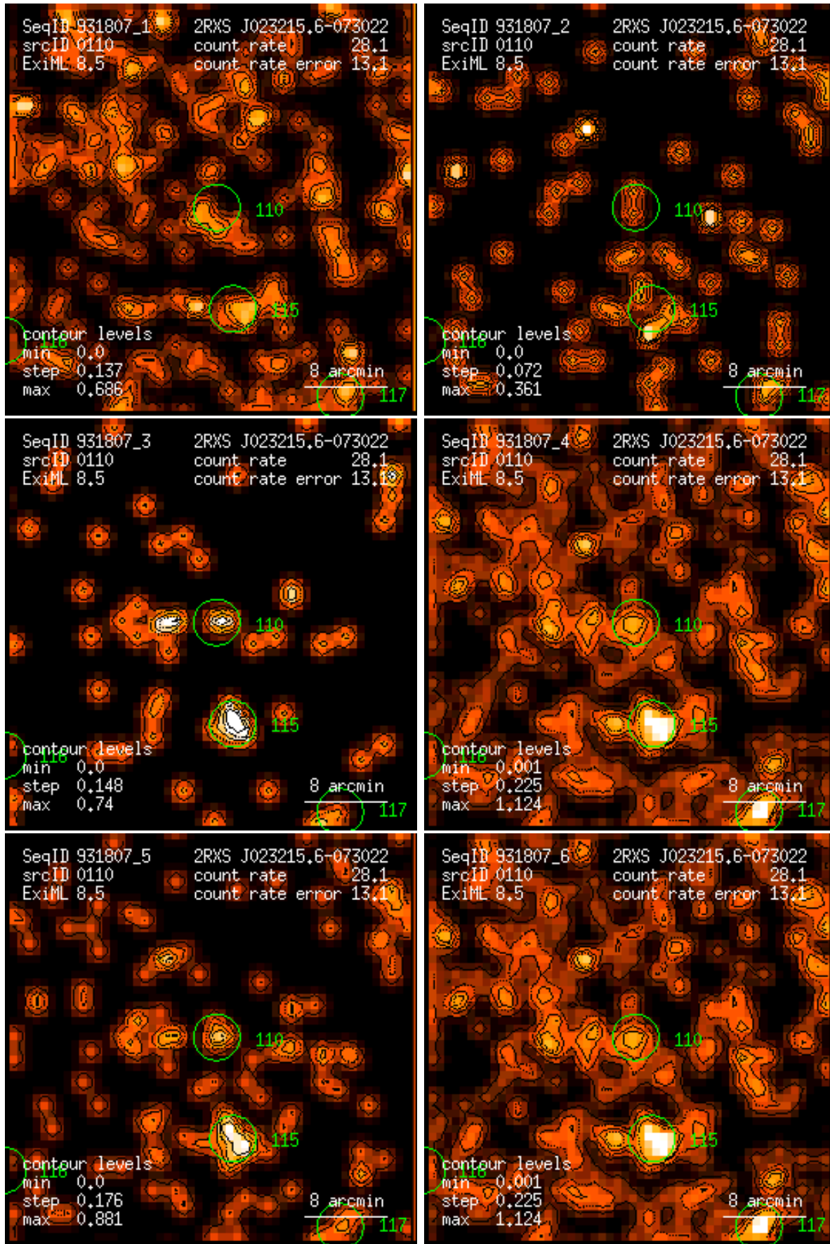
Figure 110: RASS 931807: detection 0110: band rate images, Gaussian filter: (1) PSPC channels 11 – 41, (2) 52 – 90, (3) 91 – 201, (4) 11 – 235, (5) 52 – 201, (6) 11 – 201. Broad band rates in counts/ks. Band rate contour levels in counts/ks/arcmin 2 .
