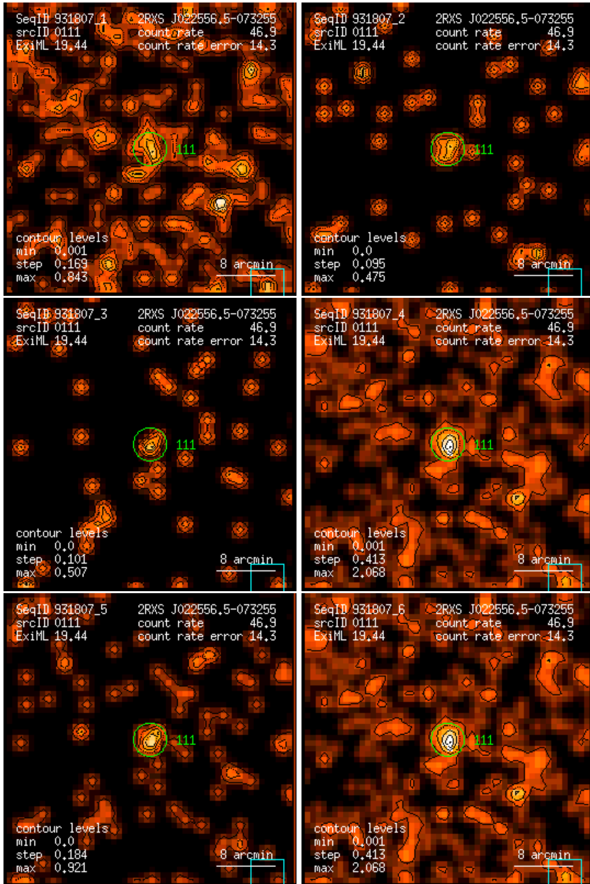
Figure 111: RASS 931807: detection 0111: band rate images, Gaussian filter: (1) PSPC channels 11 – 41, (2) 52 – 90, (3) 91 – 201, (4) 11 – 235, (5) 52 – 201, (6) 11 – 201. Broad band rates in counts/ks. Band rate contour levels in counts/ks/arcmin 2 .
