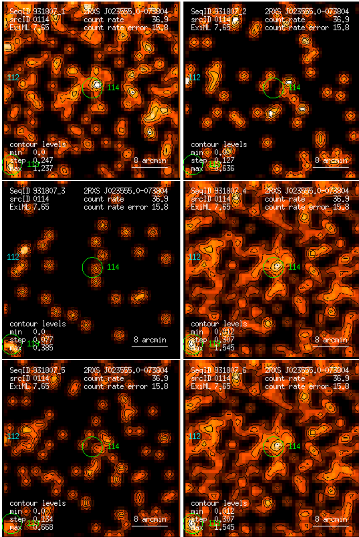
Figure 114: RASS 931807: detection 0114: band rate images, Gaussian filter: (1) PSPC channels 11 – 41, (2) 52 – 90, (3) 91 – 201, (4) 11 – 235, (5) 52 – 201, (6) 11 – 201. Broad band rates in counts/ks. Band rate contour levels in counts/ks/arcmin 2 .
