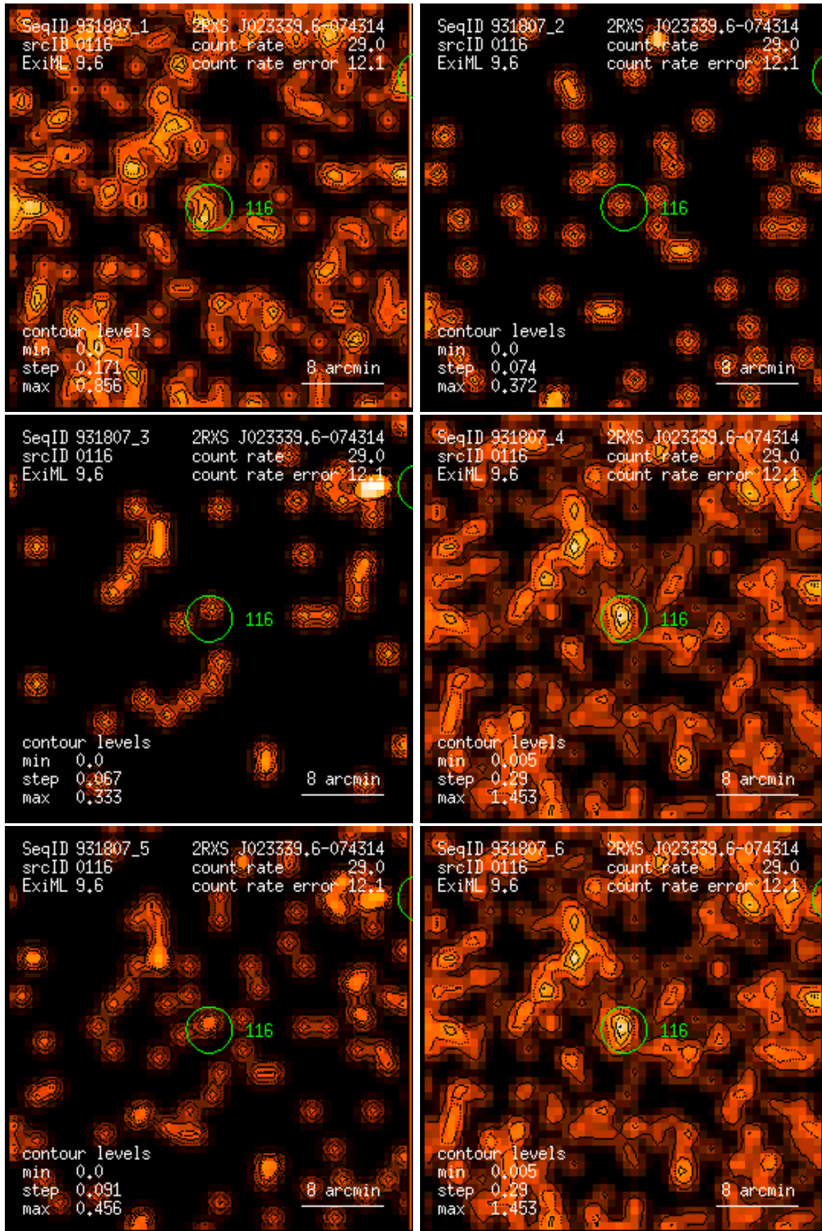
Figure 116: RASS 931807: detection 0116: band rate images, Gaussian filter: (1) PSPC channels 11 – 41, (2) 52 – 90, (3) 91 – 201, (4) 11 – 235, (5) 52 – 201, (6) 11 – 201. Broad band rates in counts/ks. Band rate contour levels in counts/ks/arcmin 2 .
