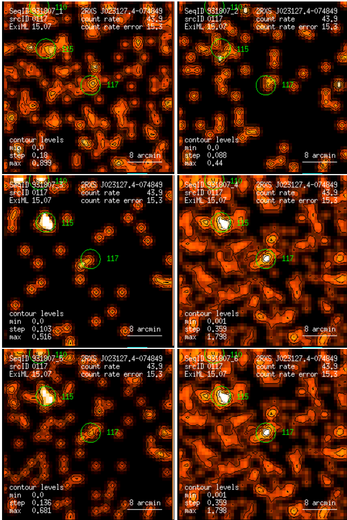
Figure 117: RASS 931807: detection 0117: band rate images, Gaussian filter: (1) PSPC channels 11 – 41, (2) 52 – 90, (3) 91 – 201, (4) 11 – 235, (5) 52 – 201, (6) 11 – 201. Broad band rates in counts/ks. Band rate contour levels in counts/ks/arcmin 2 .
