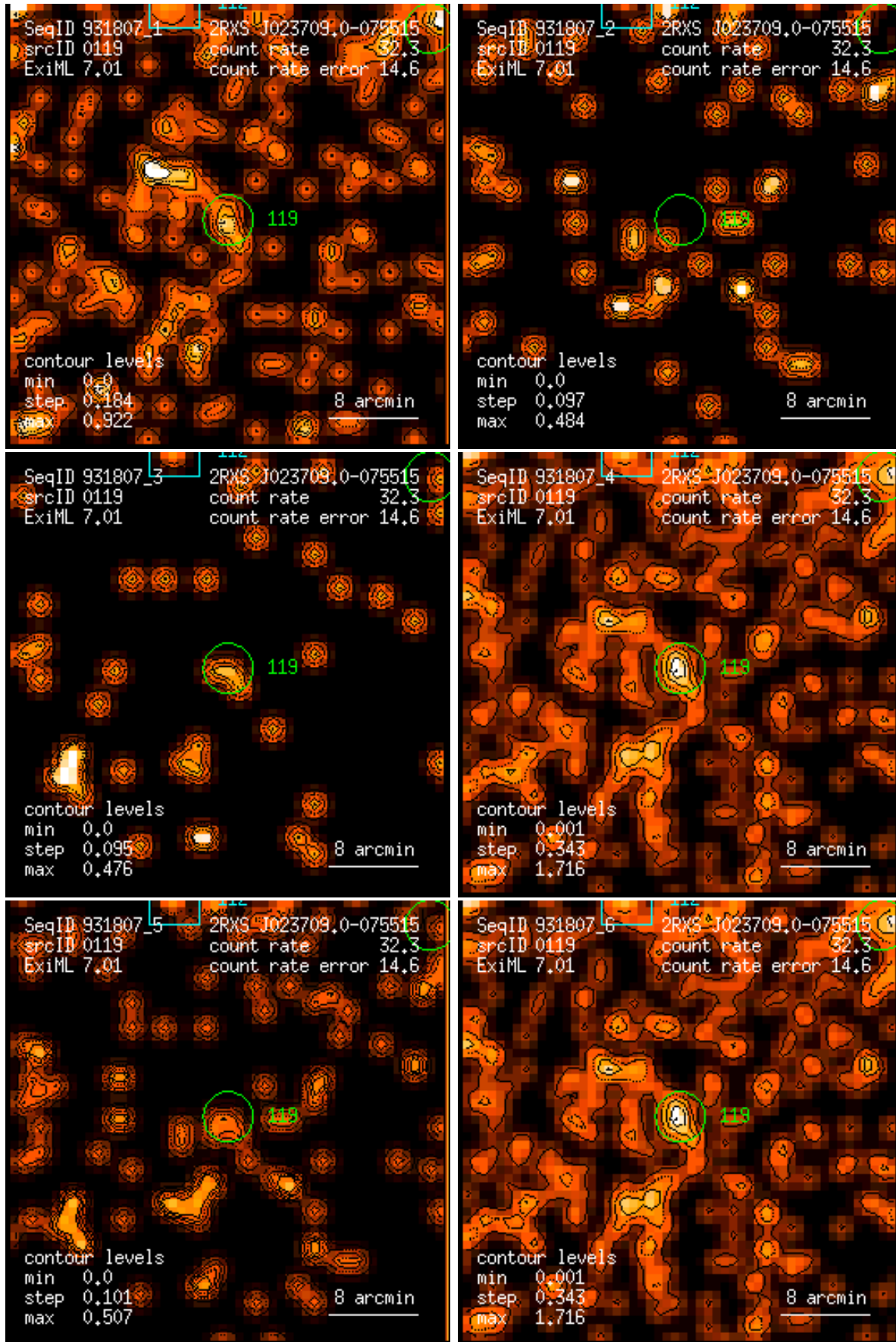
Figure 119: RASS 931807: detection 0119: band rate images, Gaussian filter: (1) PSPC channels 11 – 41, (2) 52 – 90, (3) 91 – 201, (4) 11 – 235, (5) 52 – 201, (6) 11 – 201. Broad band rates in counts/ks. Band rate contour levels in counts/ks/arcmin 2 .
