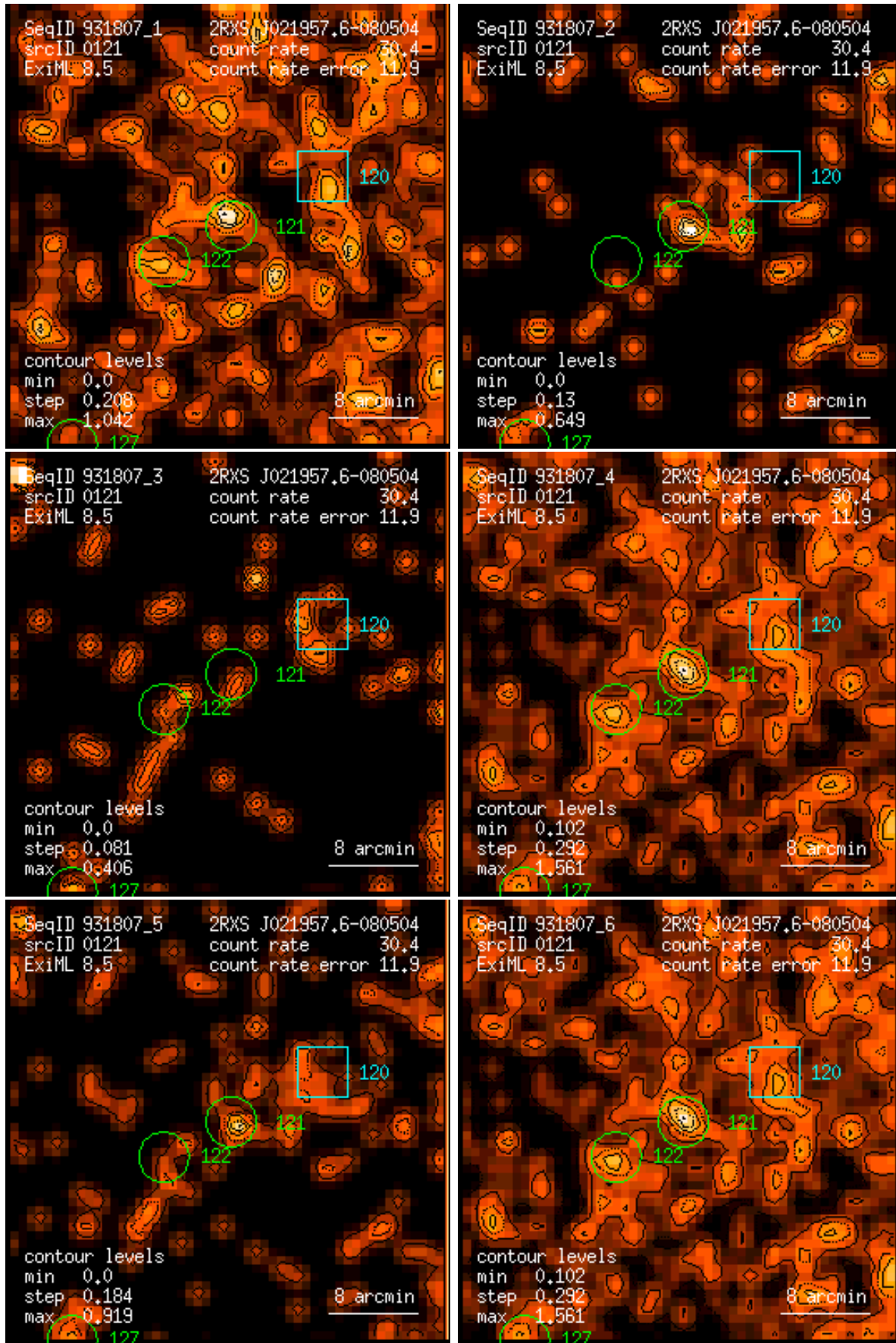
Figure 121: RASS 931807: detection 0121: band rate images, Gaussian filter: (1) PSPC channels 11 – 41, (2) 52 – 90, (3) 91 – 201, (4) 11 – 235, (5) 52 – 201, (6) 11 – 201. Broad band rates in counts/ks. Band rate contour levels in counts/ks/arcmin 2 .
