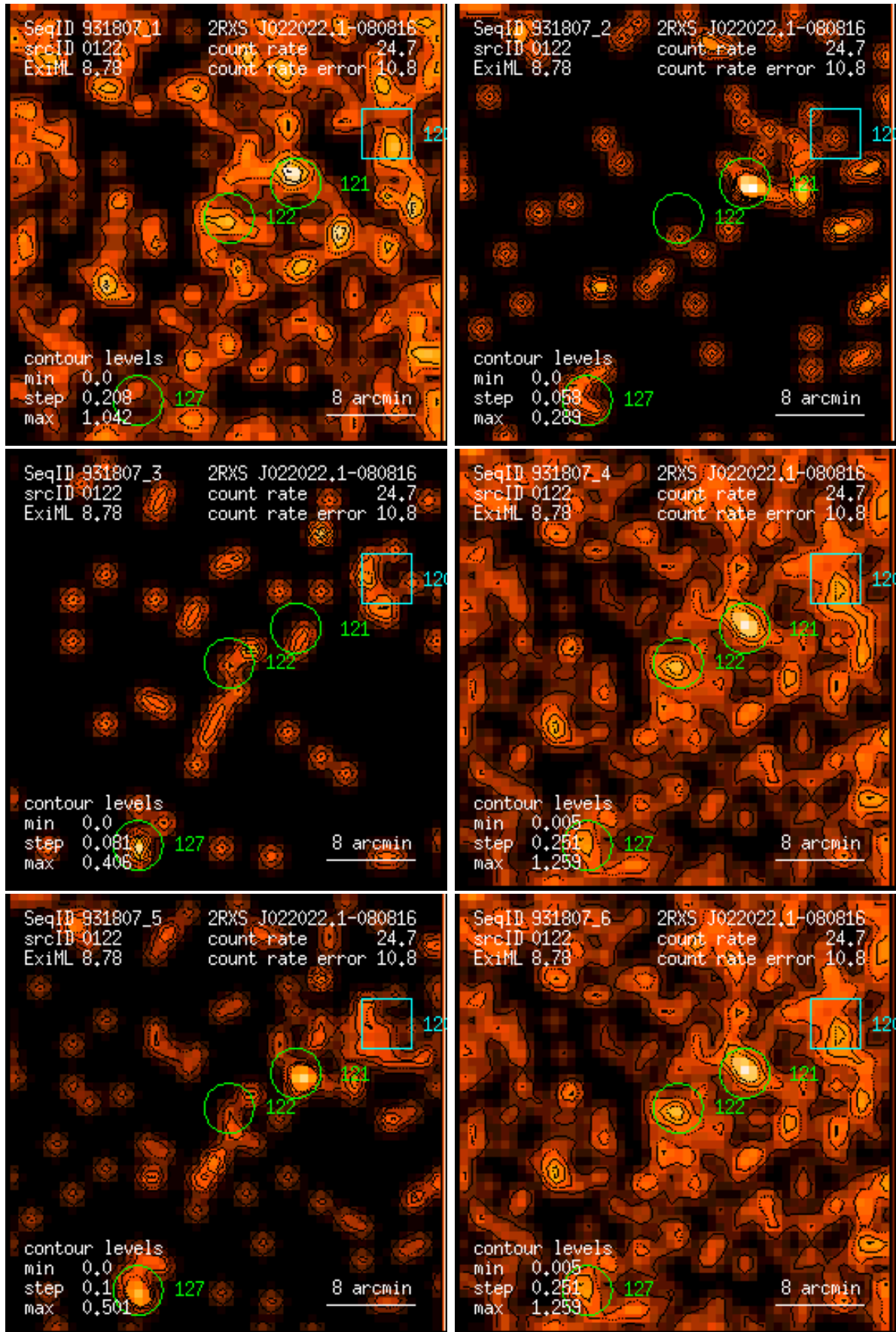
Figure 122: RASS 931807: detection 0122: band rate images, Gaussian filter: (1) PSPC channels 11 – 41, (2) 52 – 90, (3) 91 – 201, (4) 11 – 235, (5) 52 – 201, (6) 11 – 201. Broad band rates in counts/ks. Band rate contour levels in counts/ks/arcmin 2 .
