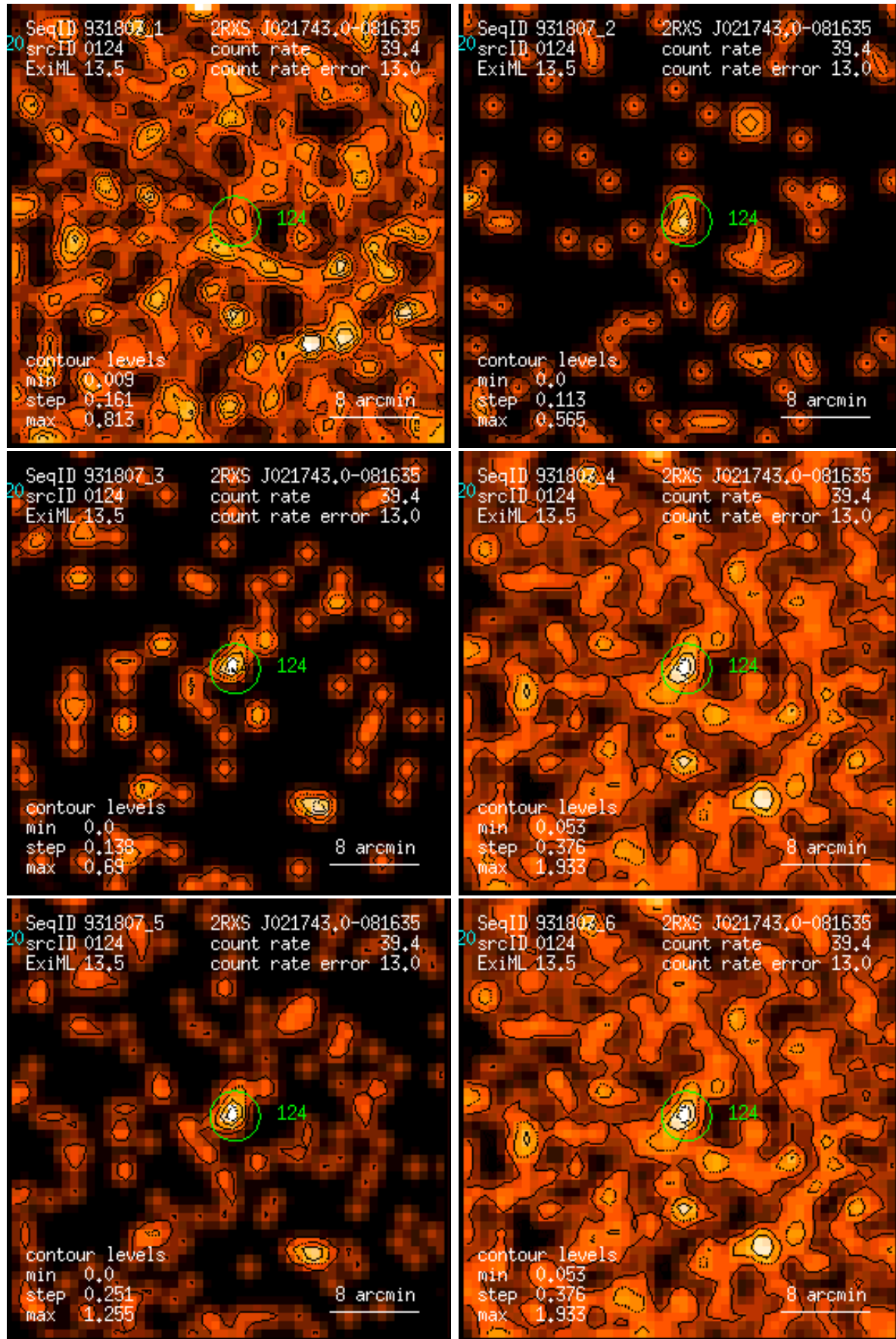
Figure 124: RASS 931807: detection 0124: band rate images, Gaussian filter: (1) PSPC channels 11 – 41, (2) 52 – 90, (3) 91 – 201, (4) 11 – 235, (5) 52 – 201, (6) 11 – 201. Broad band rates in counts/ks. Band rate contour levels in counts/ks/arcmin 2 .
