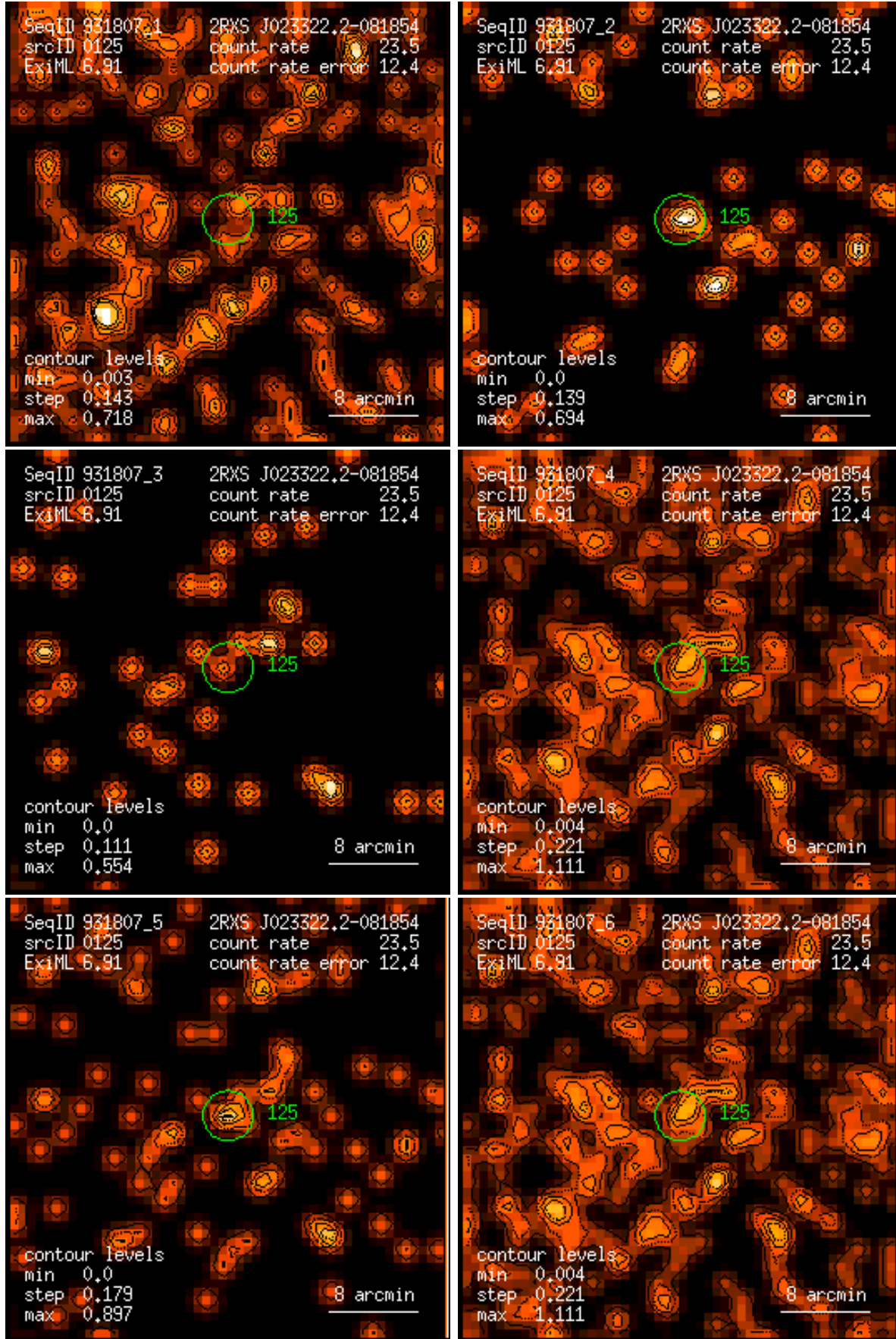
Figure 125: RASS 931807: detection 0125: band rate images, Gaussian filter: (1) PSPC channels 11 – 41, (2) 52 – 90, (3) 91 – 201, (4) 11 – 235, (5) 52 – 201, (6) 11 – 201. Broad band rates in counts/ks. Band rate contour levels in counts/ks/arcmin 2 .
