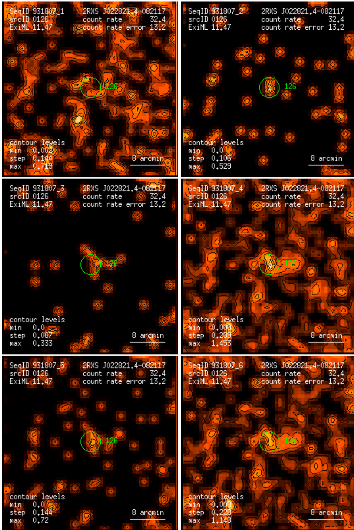
Figure 126: RASS 931807: detection 0126: band rate images, Gaussian filter: (1) PSPC channels 11 – 41, (2) 52 – 90, (3) 91 – 201, (4) 11 – 235, (5) 52 – 201, (6) 11 – 201. Broad band rates in counts/ks. Band rate contour levels in counts/ks/arcmin 2 .
