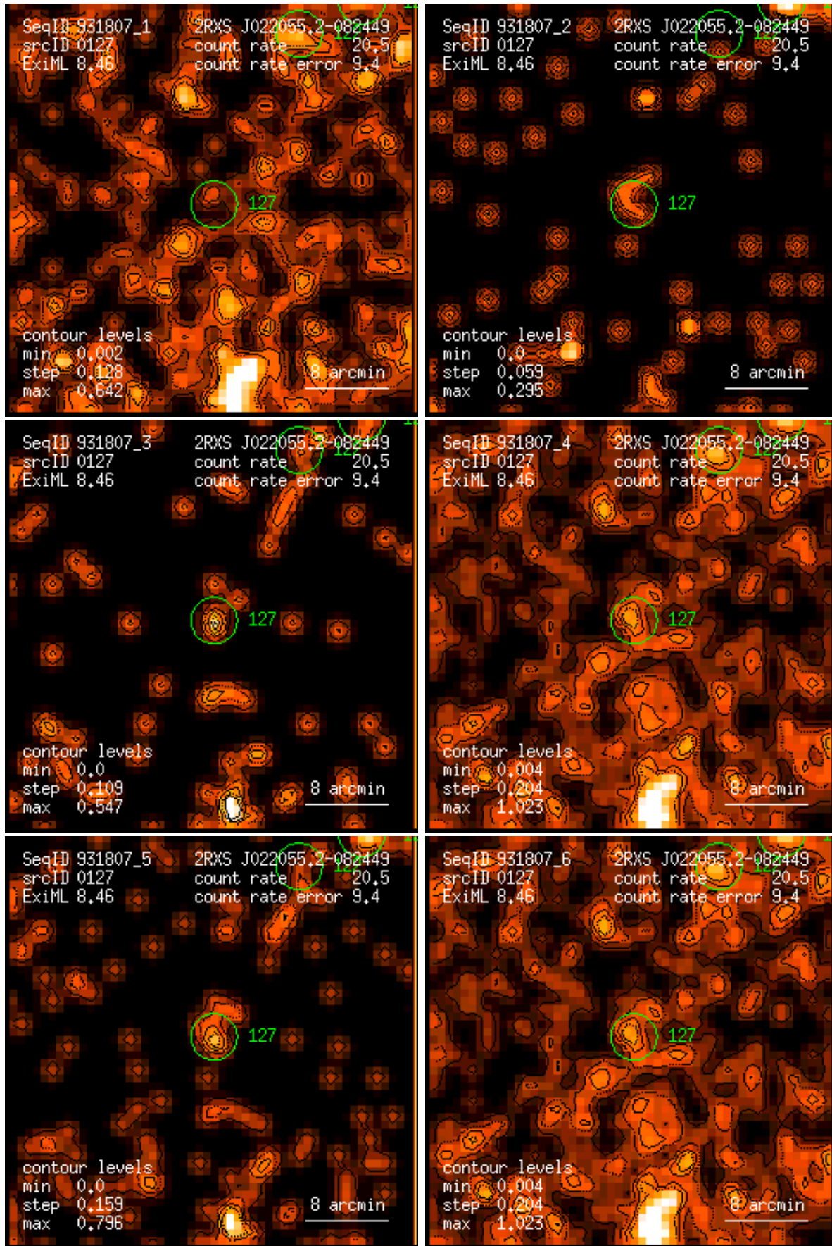
Figure 127: RASS 931807: detection 0127: band rate images, Gaussian filter: (1) PSPC channels 11 – 41, (2) 52 – 90, (3) 91 – 201, (4) 11 – 235, (5) 52 – 201, (6) 11 – 201. Broad band rates in counts/ks. Band rate contour levels in counts/ks/arcmin 2 .
