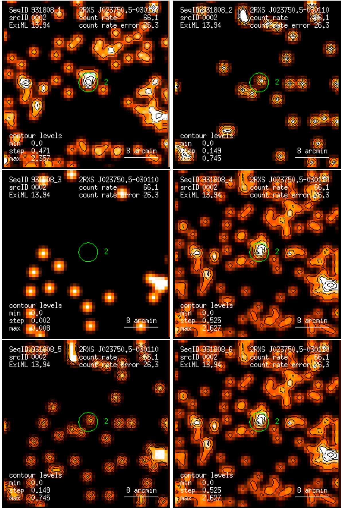
Figure 2: RASS 931808: detection 0002: band rate images, Gaussian filter: (1) PSPC channels 11 – 41, (2) 52 – 90, (3) 91 – 201, (4) 11 – 235, (5) 52 – 201, (6) 11 – 201. Broad band rates in counts/ks. Band rate contour levels in counts/ks/arcmin 2 .
