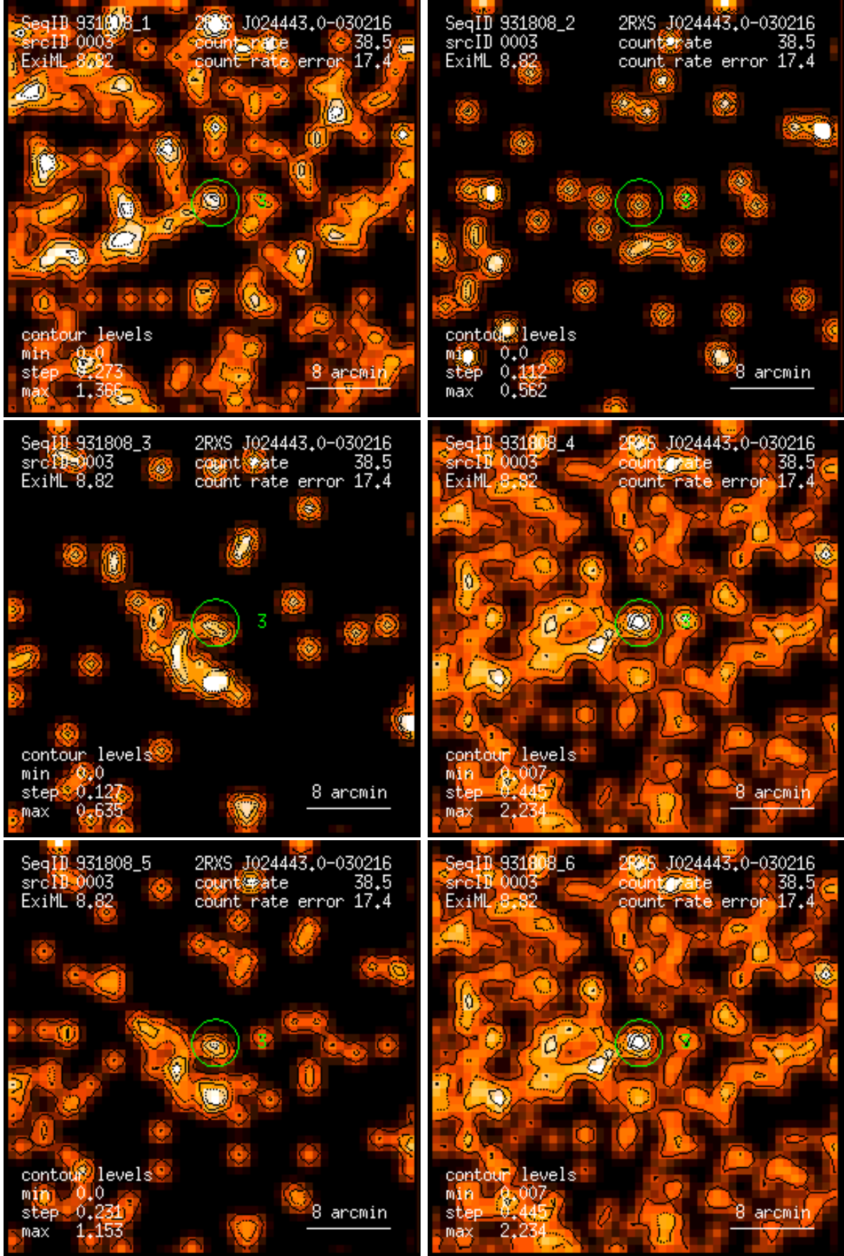
Figure 3: RASS 931808: detection 0003: band rate images, Gaussian filter: (1) PSPC channels 11 – 41, (2) 52 – 90, (3) 91 – 201, (4) 11 – 235, (5) 52 – 201, (6) 11 – 201. Broad band rates in counts/ks. Band rate contour levels in counts/ks/arcmin 2 .
