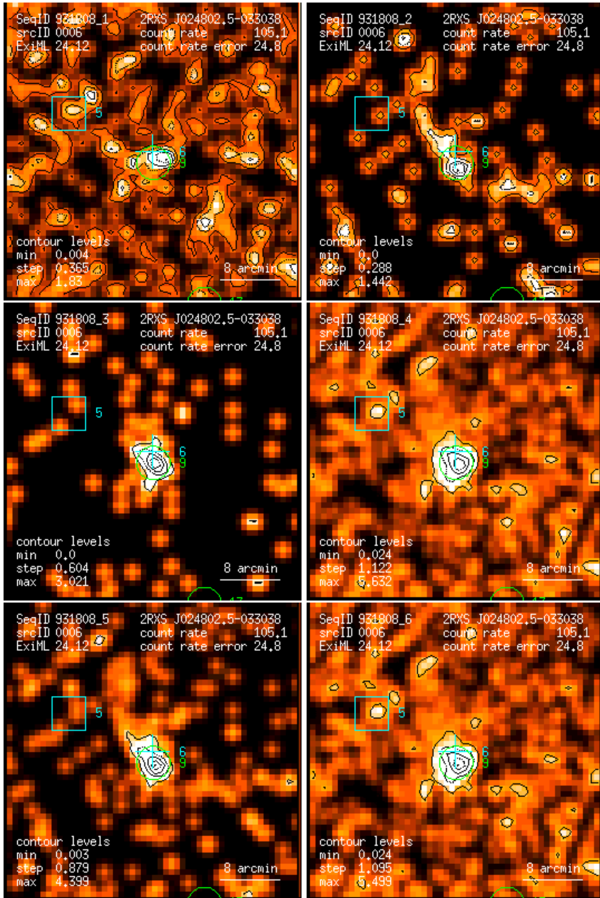
Figure 6: RASS 931808: detection 0006: band rate images, Gaussian filter: (1) PSPC channels 11 – 41, (2) 52 – 90, (3) 91 – 201, (4) 11 – 235, (5) 52 – 201, (6) 11 – 201. Broad band rates in counts/ks. Band rate contour levels in counts/ks/arcmin 2 .
