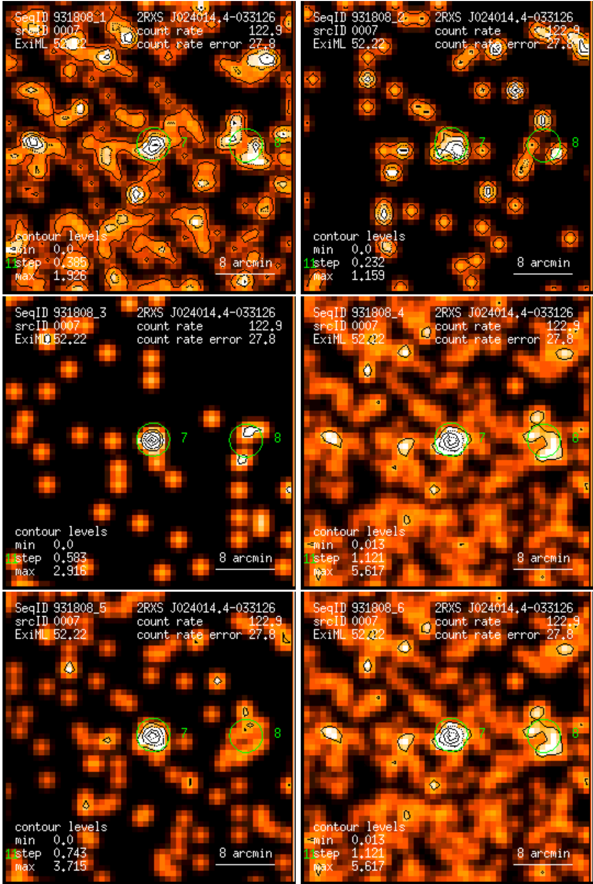
Figure 7: RASS 931808: detection 0007: band rate images, Gaussian filter: (1) PSPC channels 11 – 41, (2) 52 – 90, (3) 91 – 201, (4) 11 – 235, (5) 52 – 201, (6) 11 – 201. Broad band rates in counts/ks. Band rate contour levels in counts/ks/arcmin 2 .
