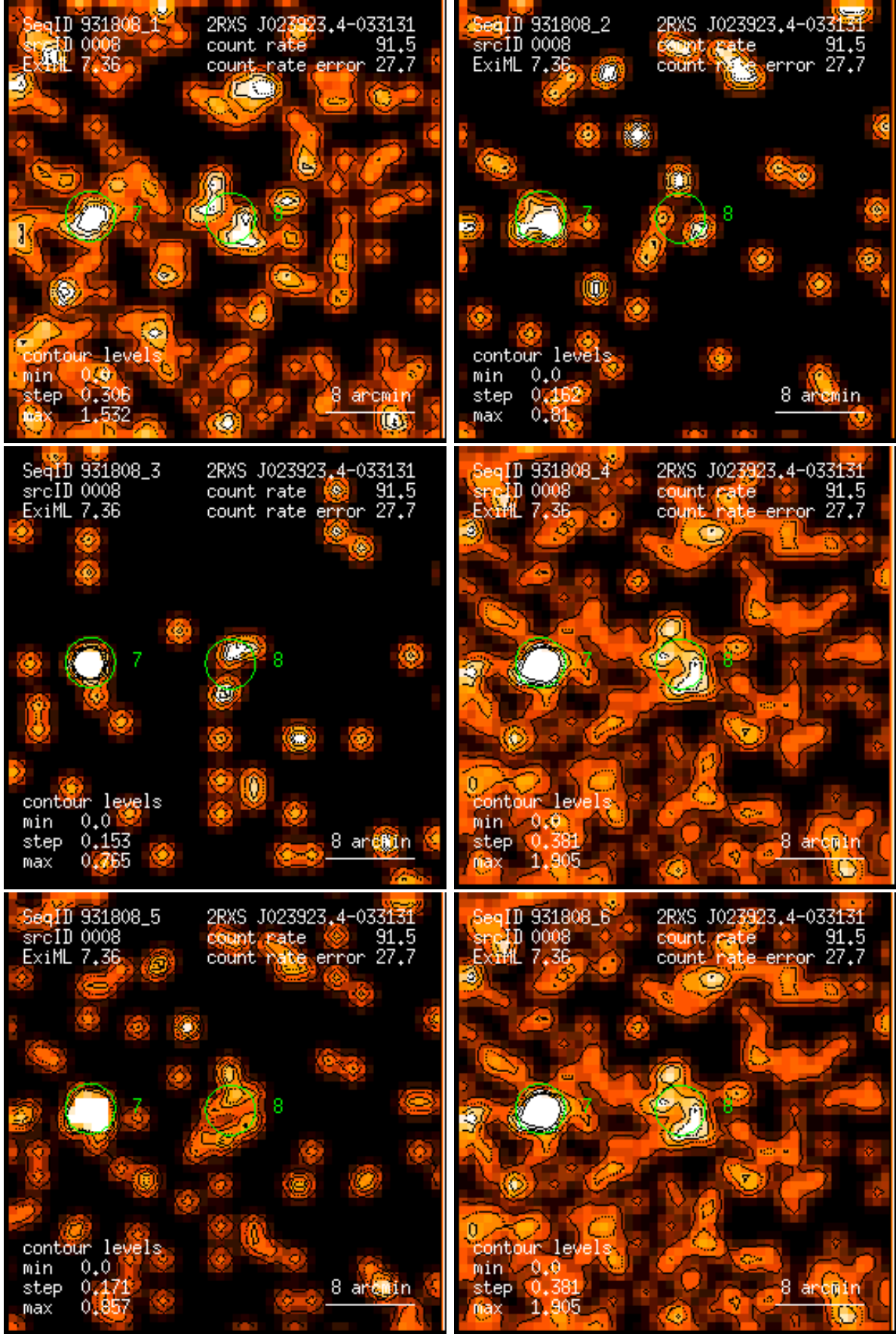
Figure 8: RASS 931808: detection 0008: band rate images, Gaussian filter: (1) PSPC channels 11 – 41, (2) 52 – 90, (3) 91 – 201, (4) 11 – 235, (5) 52 – 201, (6) 11 – 201. Broad band rates in counts/ks. Band rate contour levels in counts/ks/arcmin 2 .
