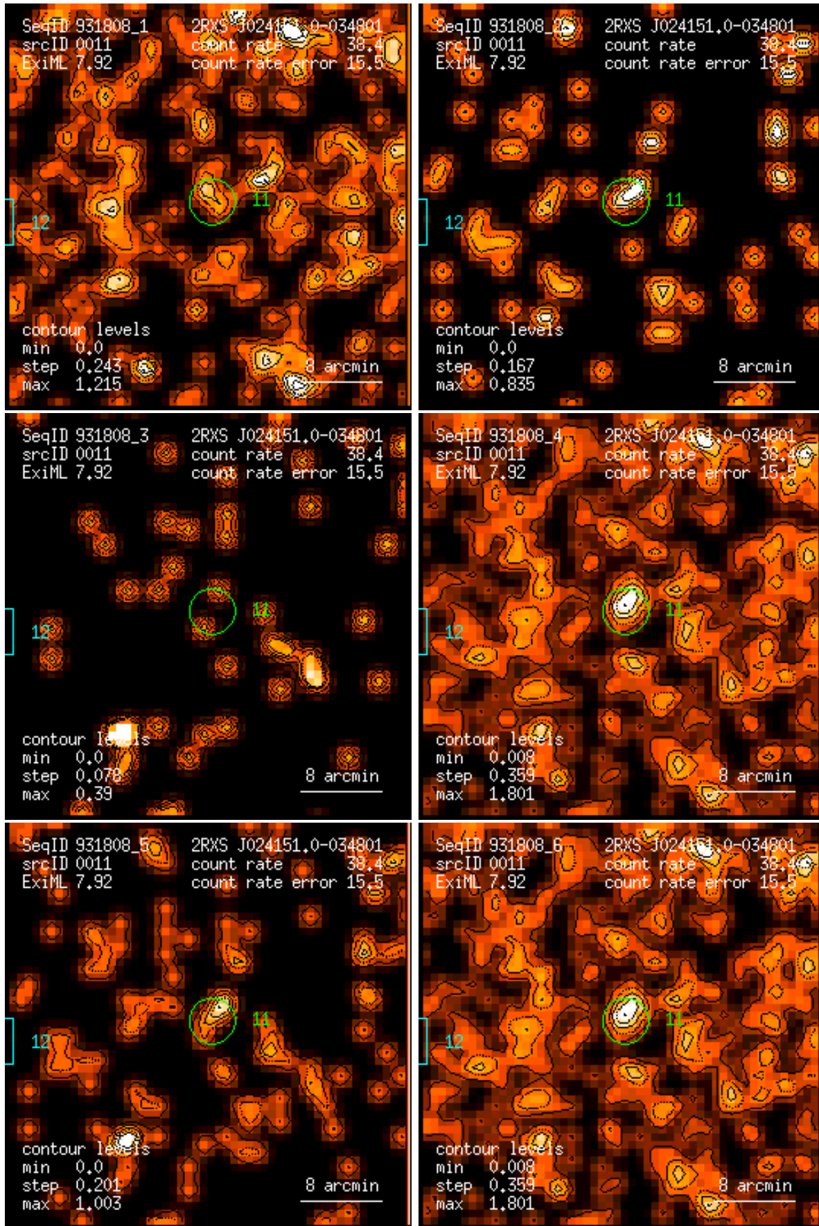
Figure 11: RASS 931808: detection 0011: band rate images, Gaussian filter: (1) PSPC channels 11 – 41, (2) 52 – 90, (3) 91 – 201, (4) 11 – 235, (5) 52 – 201, (6) 11 – 201. Broad band rates in counts/ks. Band rate contour levels in counts/ks/arcmin 2 .
