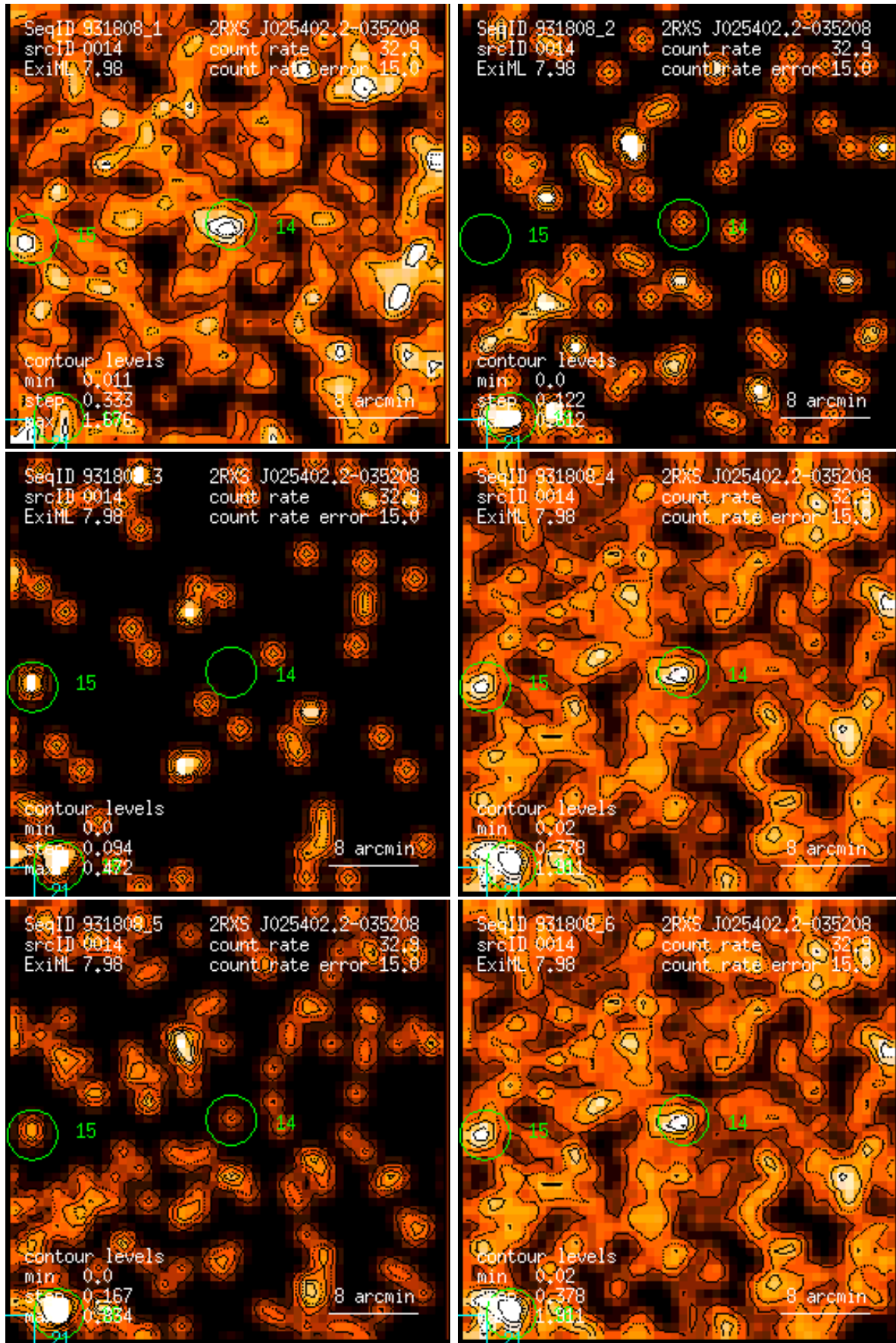
Figure 14: RASS 931808: detection 0014: band rate images, Gaussian filter: (1) PSPC channels 11 – 41, (2) 52 – 90, (3) 91 – 201, (4) 11 – 235, (5) 52 – 201, (6) 11 – 201. Broad band rates in counts/ks. Band rate contour levels in counts/ks/arcmin 2 .
