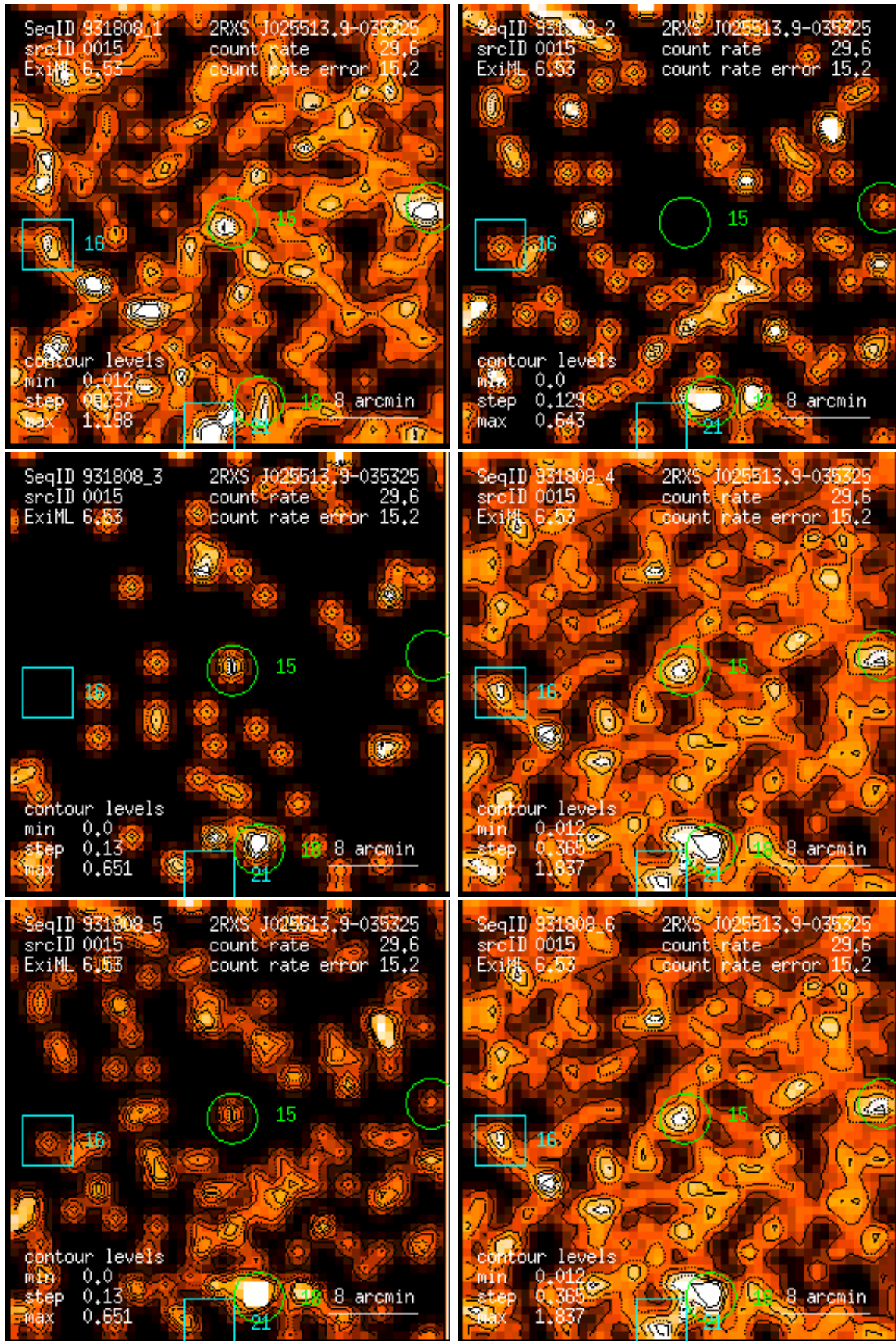
Figure 15: RASS 931808: detection 0015: band rate images, Gaussian filter: (1) PSPC channels 11 – 41, (2) 52 – 90, (3) 91 – 201, (4) 11 – 235, (5) 52 – 201, (6) 11 – 201. Broad band rates in counts/ks. Band rate contour levels in counts/ks/arcmin 2 .
