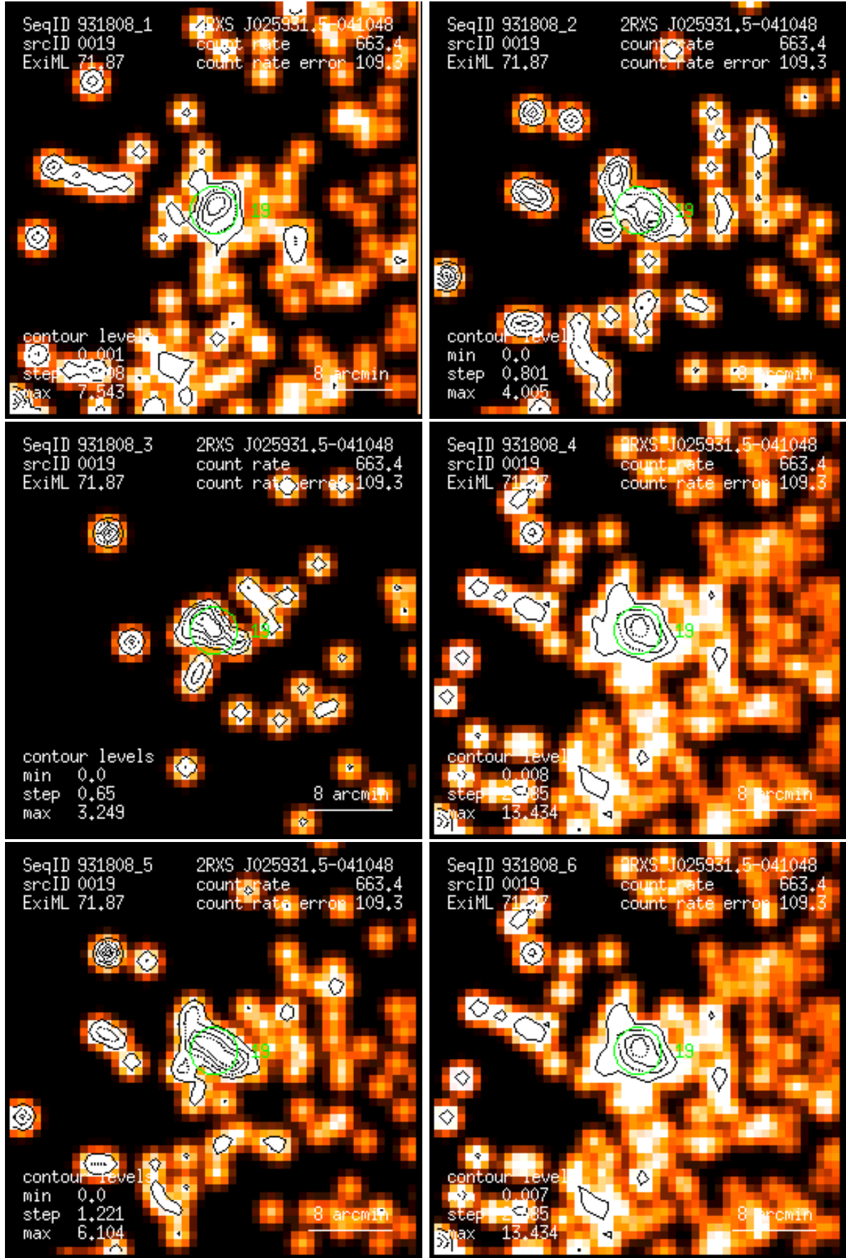
Figure 19: RASS 931808: detection 0019: band rate images, Gaussian filter: (1) PSPC channels 11 – 41, (2) 52 – 90, (3) 91 – 201, (4) 11 – 235, (5) 52 – 201, (6) 11 – 201. Broad band rates in counts/ks. Band rate contour levels in counts/ks/arcmin 2 .
