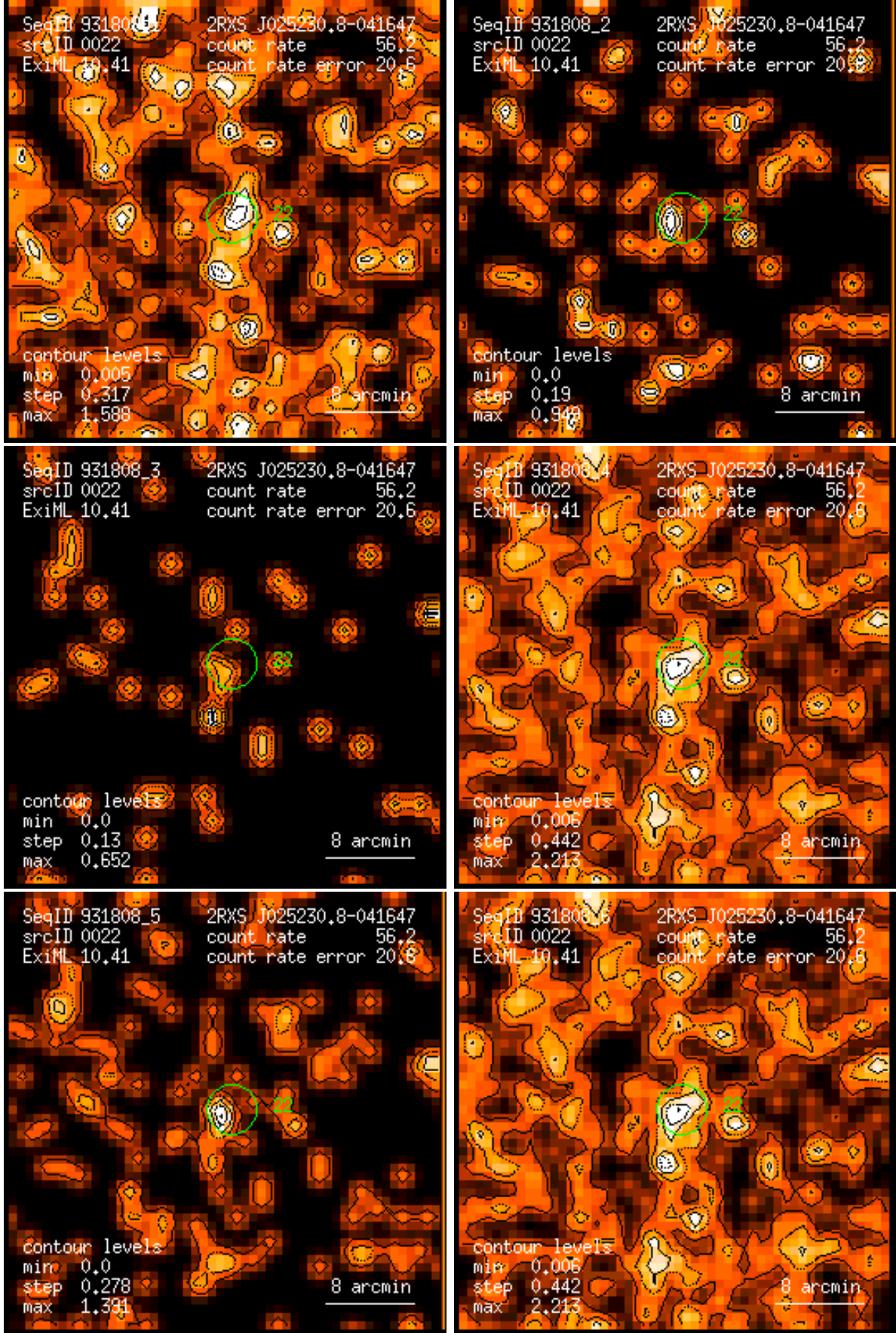
Figure 22: RASS 931808: detection 0022: band rate images, Gaussian filter: (1) PSPC channels 11 – 41, (2) 52 – 90, (3) 91 – 201, (4) 11 – 235, (5) 52 – 201, (6) 11 – 201. Broad band rates in counts/ks. Band rate contour levels in counts/ks/arcmin 2 .
