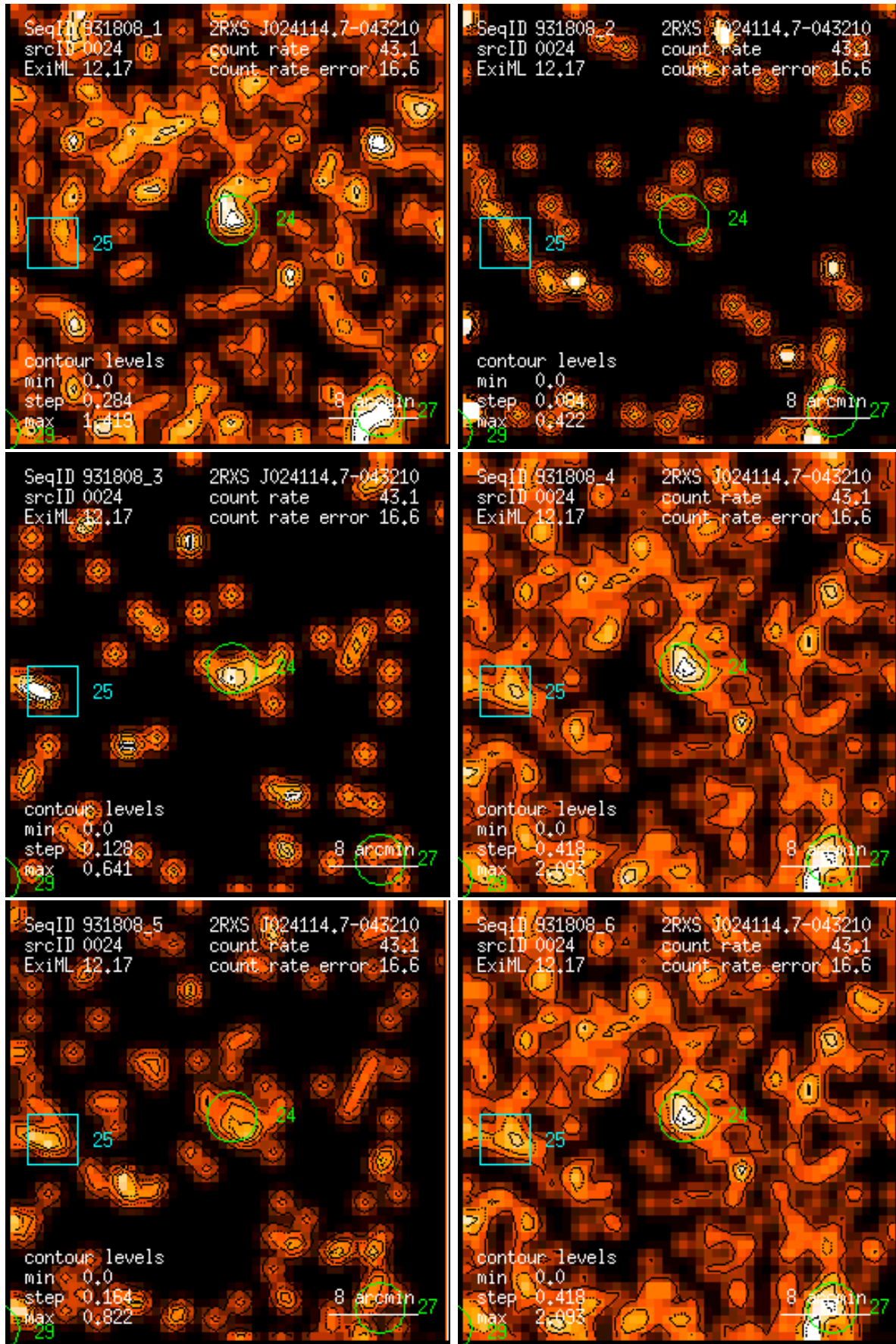
Figure 24: RASS 931808: detection 0024: band rate images, Gaussian filter: (1) PSPC channels 11 – 41, (2) 52 – 90, (3) 91 – 201, (4) 11 – 235, (5) 52 – 201, (6) 11 – 201. Broad band rates in counts/ks. Band rate contour levels in counts/ks/arcmin 2 .
