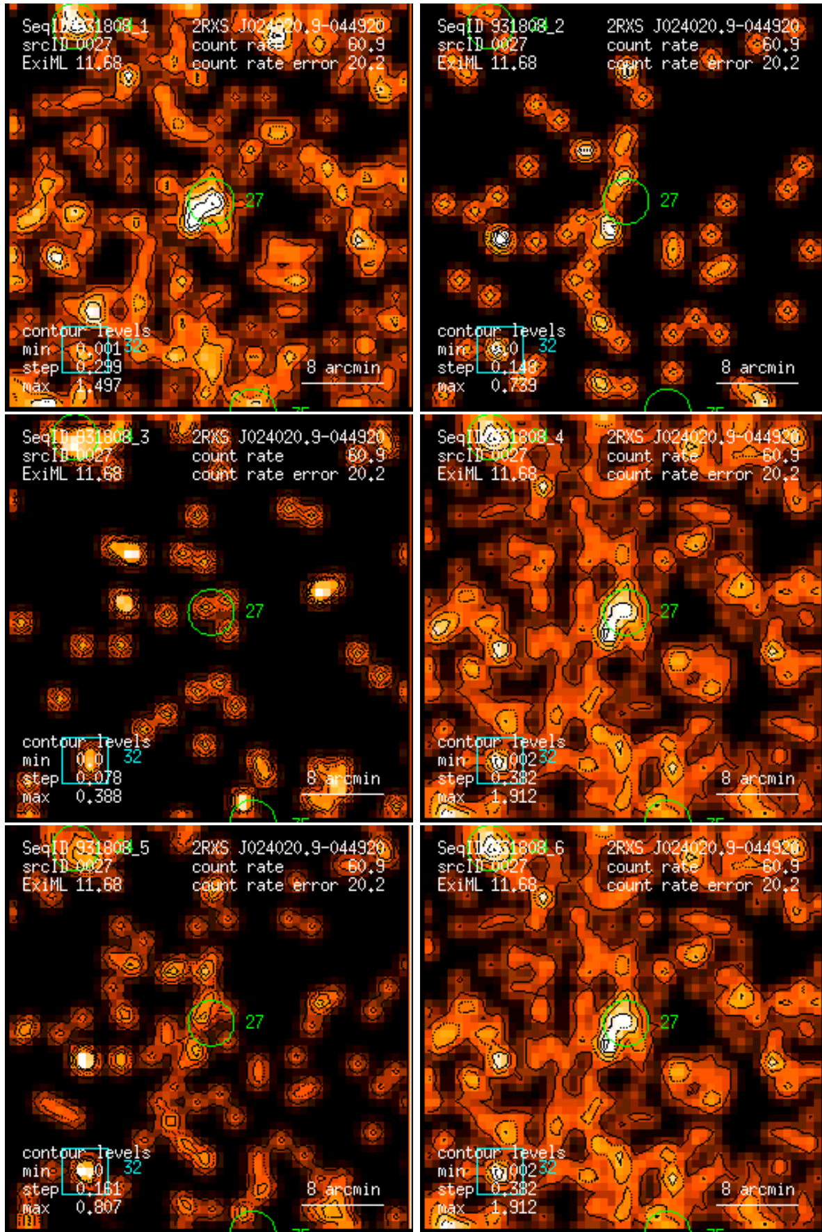
Figure 27: RASS 931808: detection 0027: band rate images, Gaussian filter: (1) PSPC channels 11 – 41, (2) 52 – 90, (3) 91 – 201, (4) 11 – 235, (5) 52 – 201, (6) 11 – 201. Broad band rates in counts/ks. Band rate contour levels in counts/ks/arcmin 2 .
