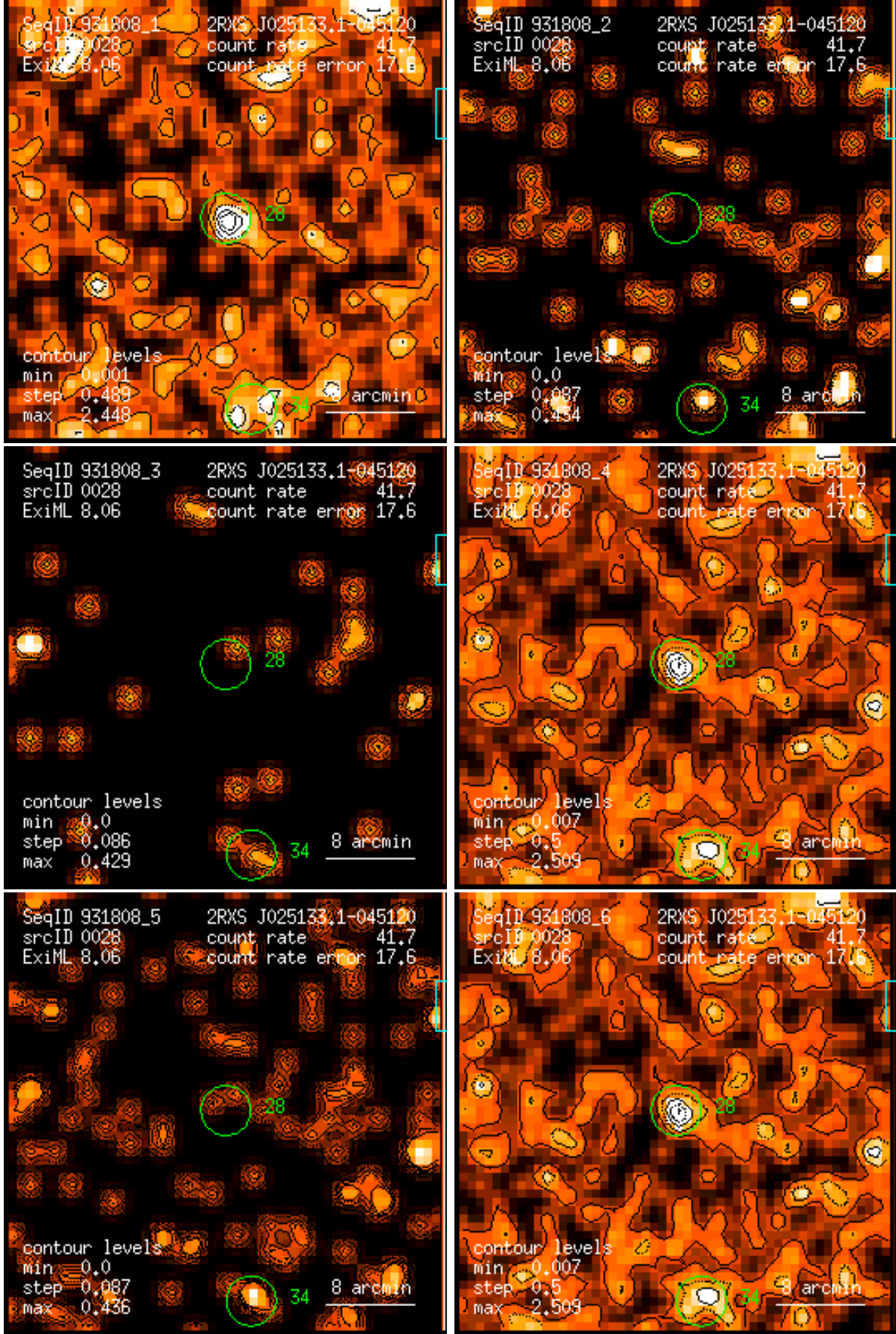
Figure 28: RASS 931808: detection 0028: band rate images, Gaussian filter: (1) PSPC channels 11 – 41, (2) 52 – 90, (3) 91 – 201, (4) 11 – 235, (5) 52 – 201, (6) 11 – 201. Broad band rates in counts/ks. Band rate contour levels in counts/ks/arcmin 2 .
