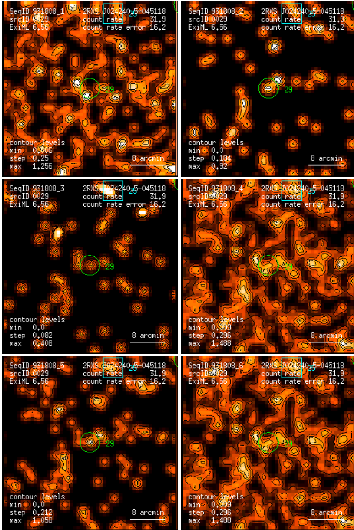
Figure 29: RASS 931808: detection 0029: band rate images, Gaussian filter: (1) PSPC channels 11 – 41, (2) 52 – 90, (3) 91 – 201, (4) 11 – 235, (5) 52 – 201, (6) 11 – 201. Broad band rates in counts/ks. Band rate contour levels in counts/ks/arcmin 2 .
