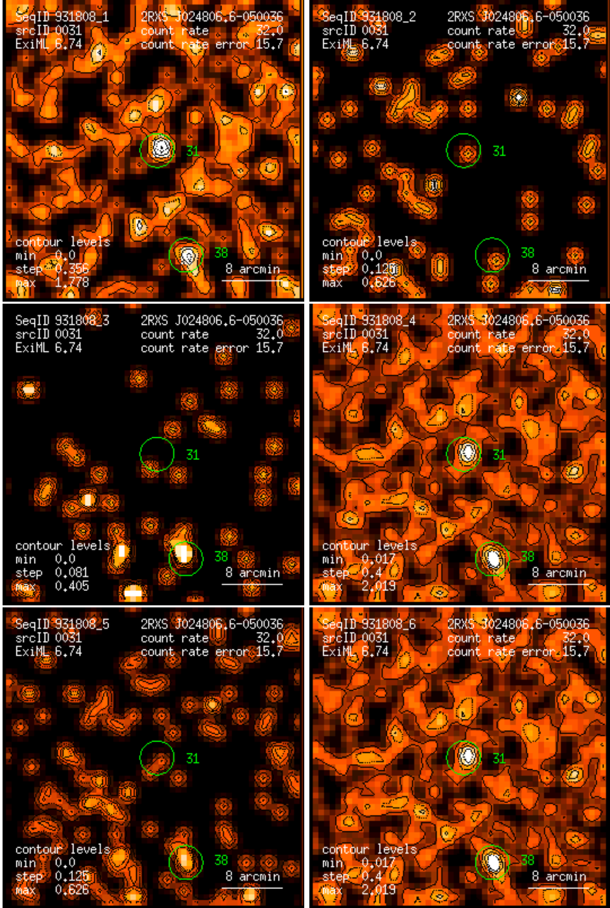
Figure 31: RASS 931808: detection 0031: band rate images, Gaussian filter: (1) PSPC channels 11 – 41, (2) 52 – 90, (3) 91 – 201, (4) 11 – 235, (5) 52 – 201, (6) 11 – 201. Broad band rates in counts/ks. Band rate contour levels in counts/ks/arcmin 2 .
