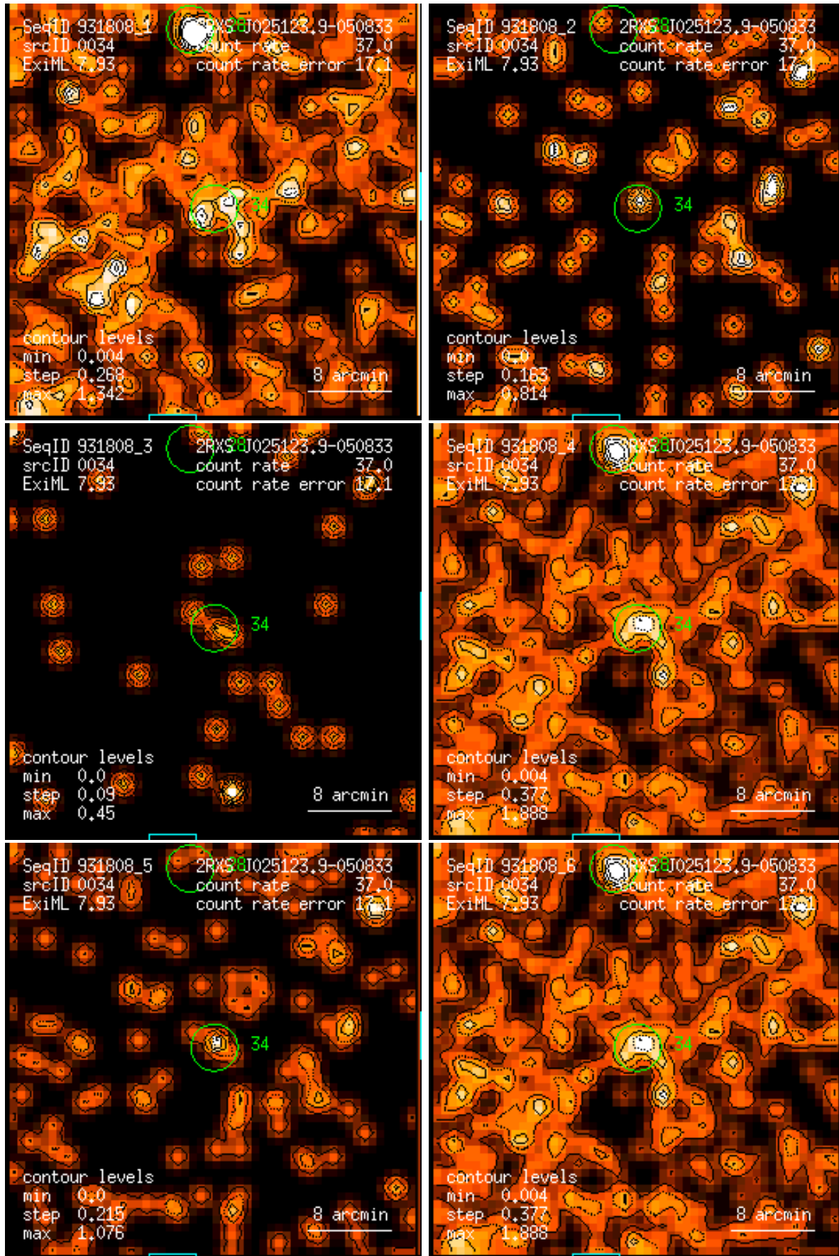
Figure 34: RASS 931808: detection 0034: band rate images, Gaussian filter: (1) PSPC channels 11 – 41, (2) 52 – 90, (3) 91 – 201, (4) 11 – 235, (5) 52 – 201, (6) 11 – 201. Broad band rates in counts/ks. Band rate contour levels in counts/ks/arcmin 2 .
