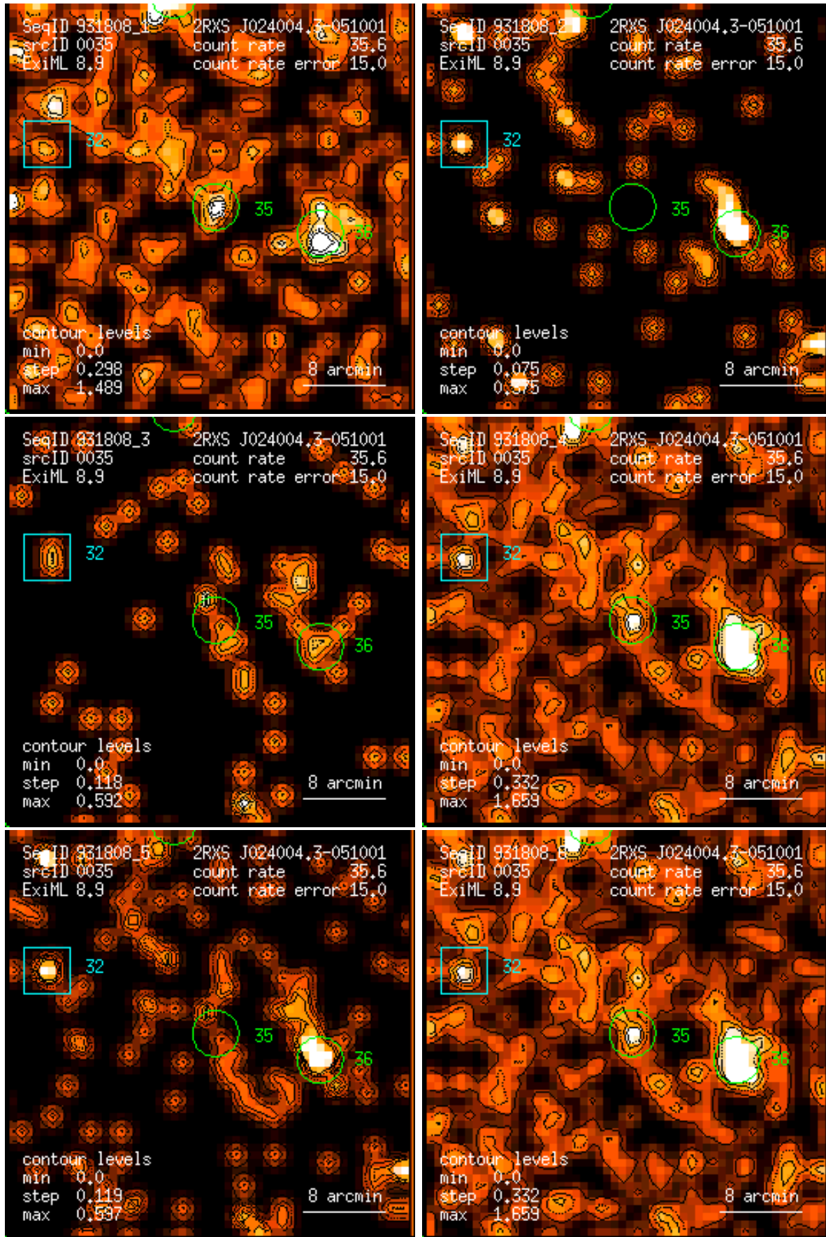
Figure 35: RASS 931808: detection 0035: band rate images, Gaussian filter: (1) PSPC channels 11 – 41, (2) 52 – 90, (3) 91 – 201, (4) 11 – 235, (5) 52 – 201, (6) 11 – 201. Broad band rates in counts/ks. Band rate contour levels in counts/ks/arcmin 2 .
