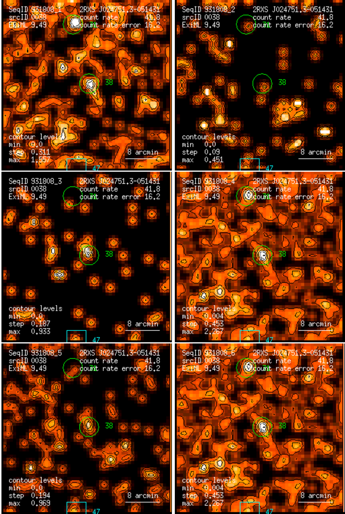
Figure 38: RASS 931808: detection 0038: band rate images, Gaussian filter: (1) PSPC channels 11 – 41, (2) 52 – 90, (3) 91 – 201, (4) 11 – 235, (5) 52 – 201, (6) 11 – 201. Broad band rates in counts/ks. Band rate contour levels in counts/ks/arcmin 2 .
