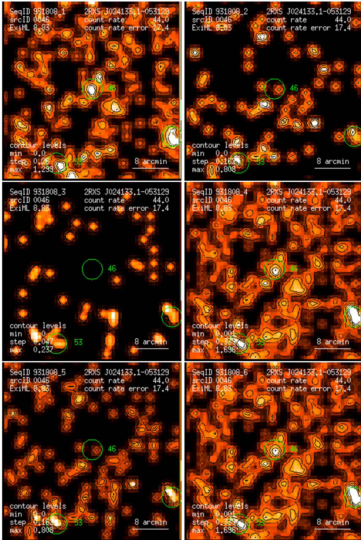
Figure 46: RASS 931808: detection 0046: band rate images, Gaussian filter: (1) PSPC channels 11 – 41, (2) 52 – 90, (3) 91 – 201, (4) 11 – 235, (5) 52 – 201, (6) 11 – 201. Broad band rates in counts/ks. Band rate contour levels in counts/ks/arcmin 2 .
