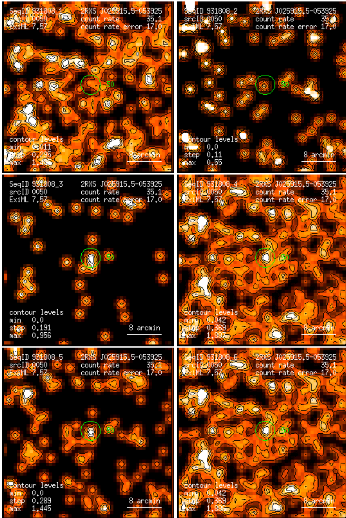
Figure 50: RASS 931808: detection 0050: band rate images, Gaussian filter: (1) PSPC channels 11 – 41, (2) 52 – 90, (3) 91 – 201, (4) 11 – 235, (5) 52 – 201, (6) 11 – 201. Broad band rates in counts/ks. Band rate contour levels in counts/ks/arcmin 2 .
