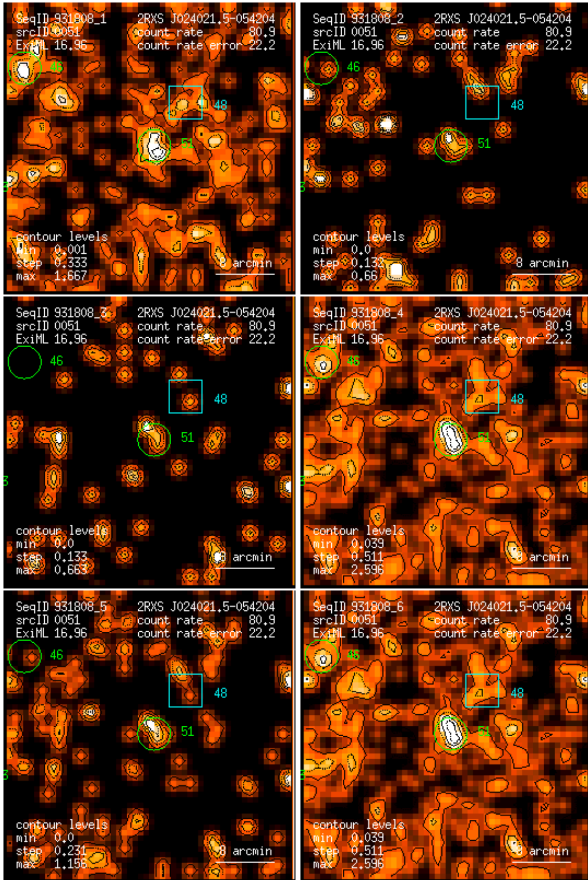
Figure 51: RASS 931808: detection 0051: band rate images, Gaussian filter: (1) PSPC channels 11 – 41, (2) 52 – 90, (3) 91 – 201, (4) 11 – 235, (5) 52 – 201, (6) 11 – 201. Broad band rates in counts/ks. Band rate contour levels in counts/ks/arcmin 2 .
