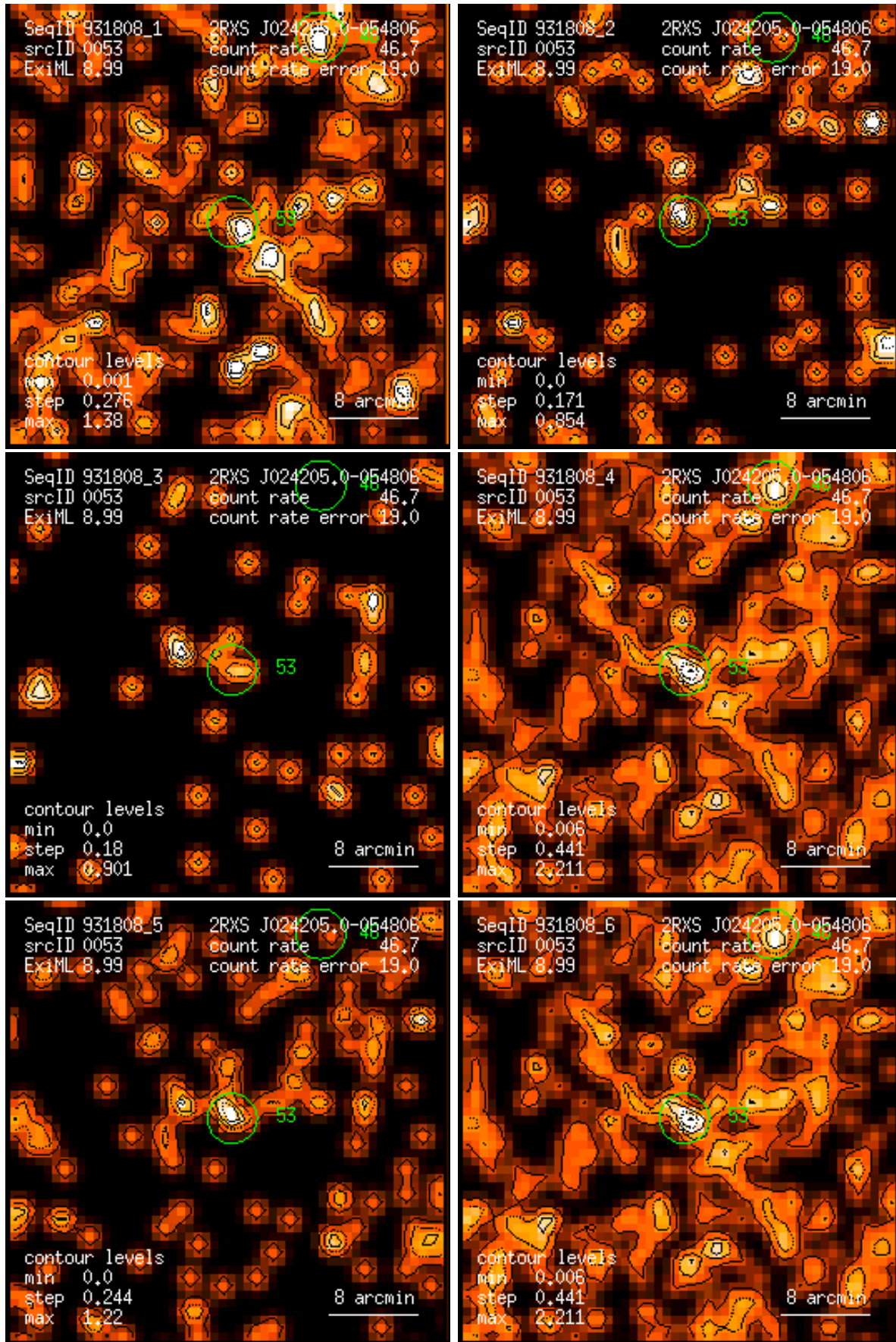
Figure 53: RASS 931808: detection 0053: band rate images, Gaussian filter: (1) PSPC channels 11 – 41, (2) 52 – 90, (3) 91 – 201, (4) 11 – 235, (5) 52 – 201, (6) 11 – 201. Broad band rates in counts/ks. Band rate contour levels in counts/ks/arcmin 2 .
