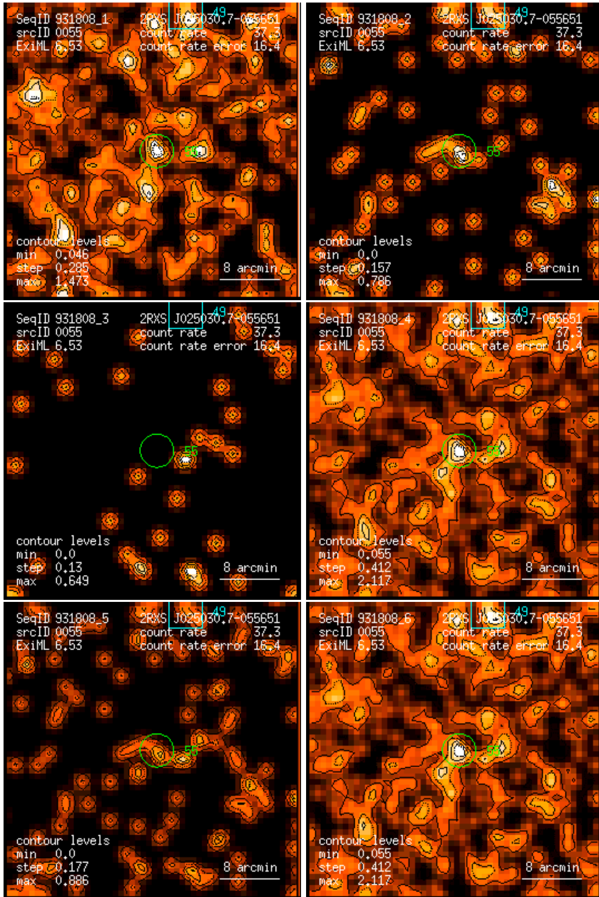
Figure 55: RASS 931808: detection 0055: band rate images, Gaussian filter: (1) PSPC channels 11 – 41, (2) 52 – 90, (3) 91 – 201, (4) 11 – 235, (5) 52 – 201, (6) 11 – 201. Broad band rates in counts/ks. Band rate contour levels in counts/ks/arcmin 2 .
