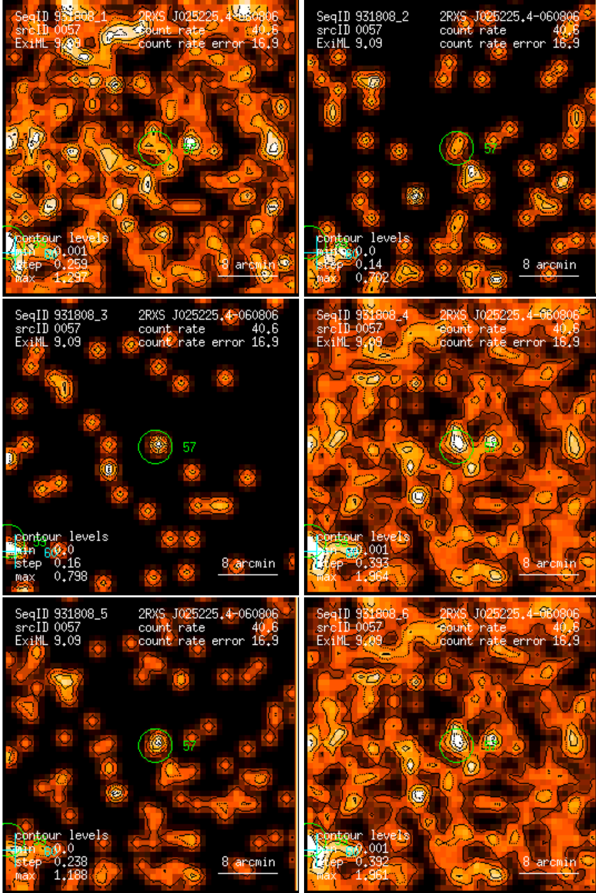
Figure 57: RASS 931808: detection 0057: band rate images, Gaussian filter: (1) PSPC channels 11 – 41, (2) 52 – 90, (3) 91 – 201, (4) 11 – 235, (5) 52 – 201, (6) 11 – 201. Broad band rates in counts/ks. Band rate contour levels in counts/ks/arcmin 2 .
