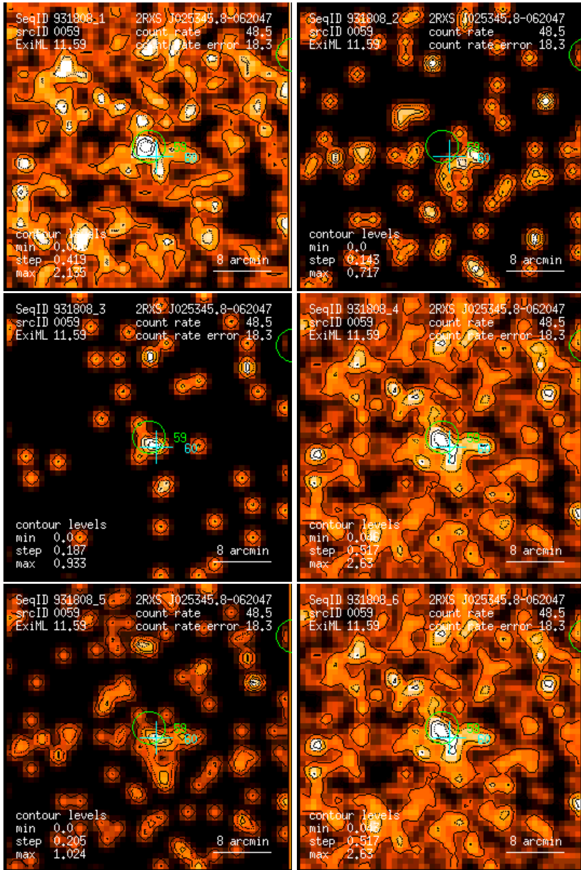
Figure 59: RASS 931808: detection 0059: band rate images, Gaussian filter: (1) PSPC channels 11 – 41, (2) 52 – 90, (3) 91 – 201, (4) 11 – 235, (5) 52 – 201, (6) 11 – 201. Broad band rates in counts/ks. Band rate contour levels in counts/ks/arcmin 2 .
