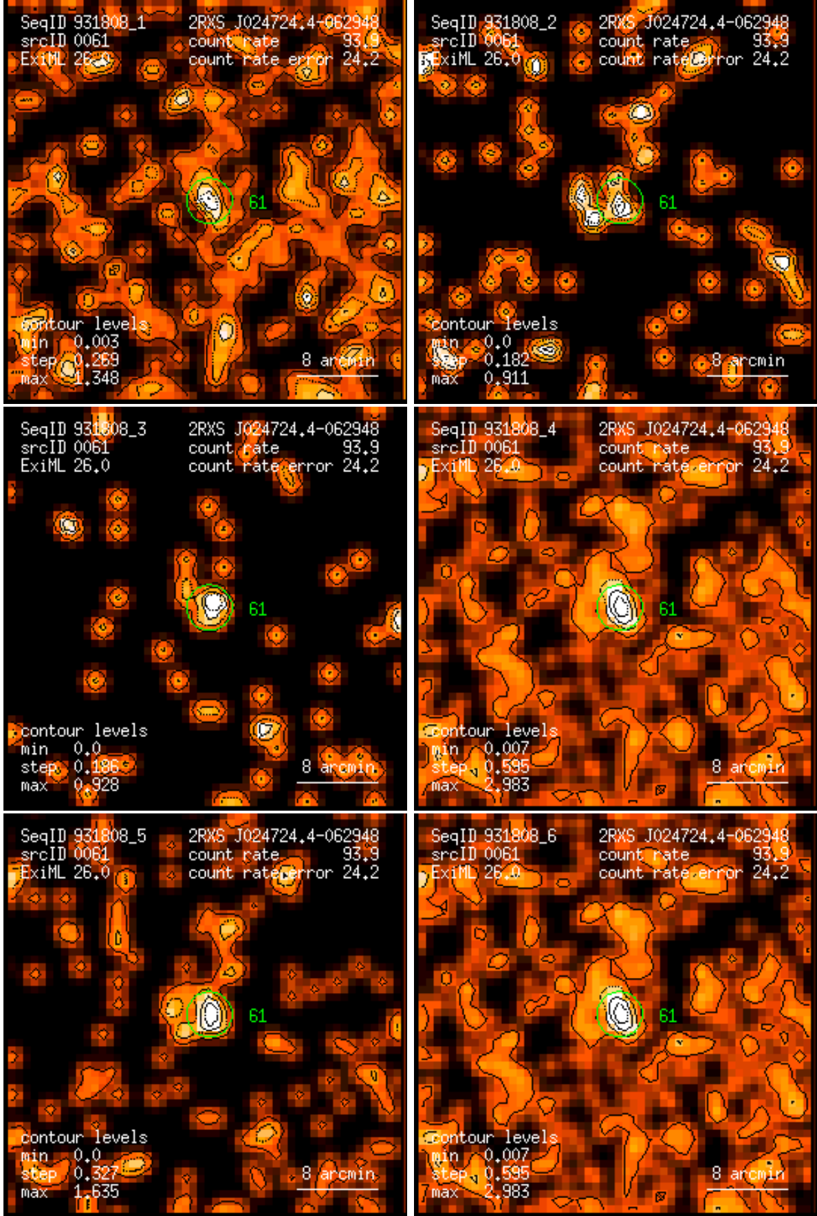
Figure 61: RASS 931808: detection 0061: band rate images, Gaussian filter: (1) PSPC channels 11 – 41, (2) 52 – 90, (3) 91 – 201, (4) 11 – 235, (5) 52 – 201, (6) 11 – 201. Broad band rates in counts/ks. Band rate contour levels in counts/ks/arcmin 2 .
