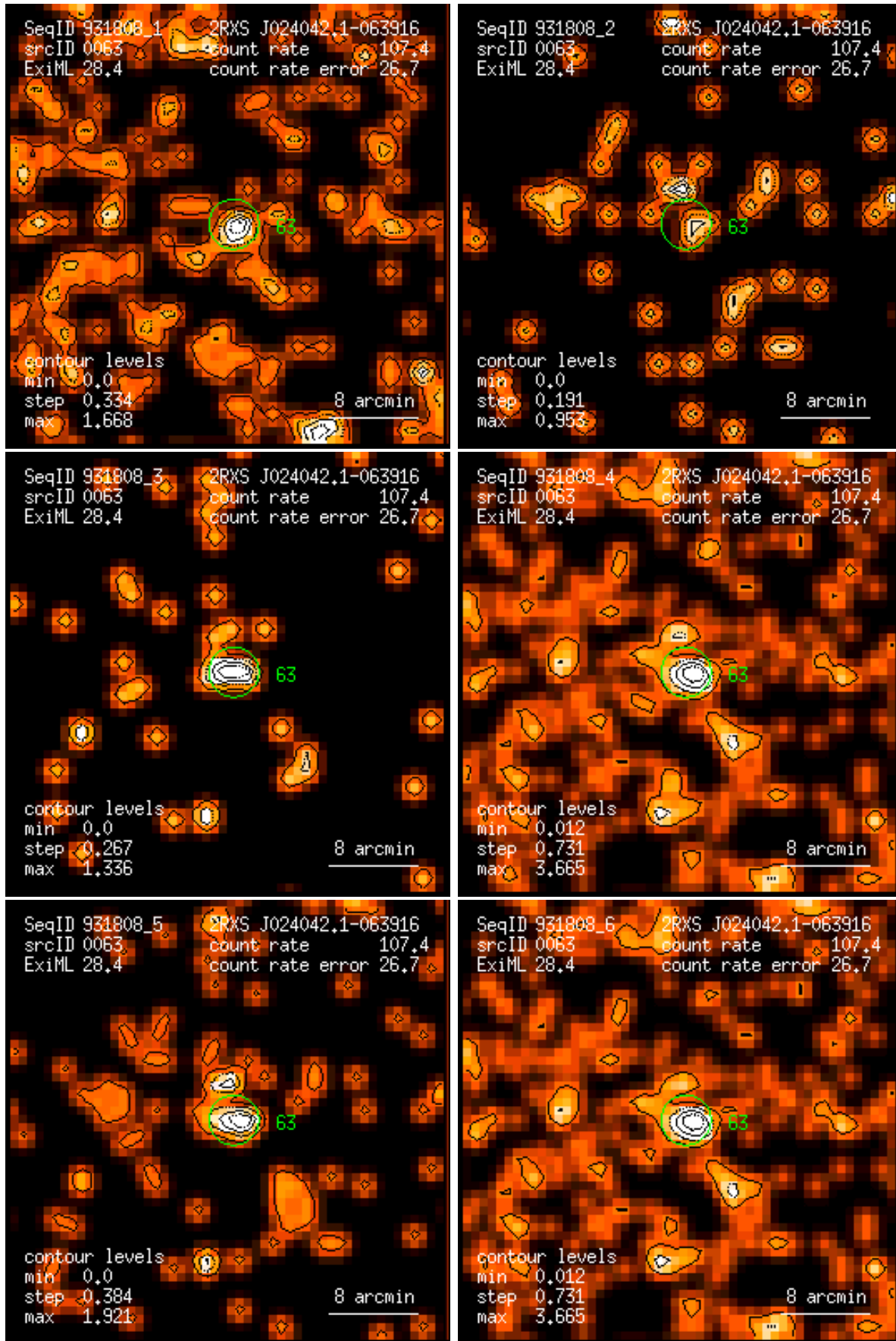
Figure 63: RASS 931808: detection 0063: band rate images, Gaussian filter: (1) PSPC channels 11 – 41, (2) 52 – 90, (3) 91 – 201, (4) 11 – 235, (5) 52 – 201, (6) 11 – 201. Broad band rates in counts/ks. Band rate contour levels in counts/ks/arcmin 2 .
